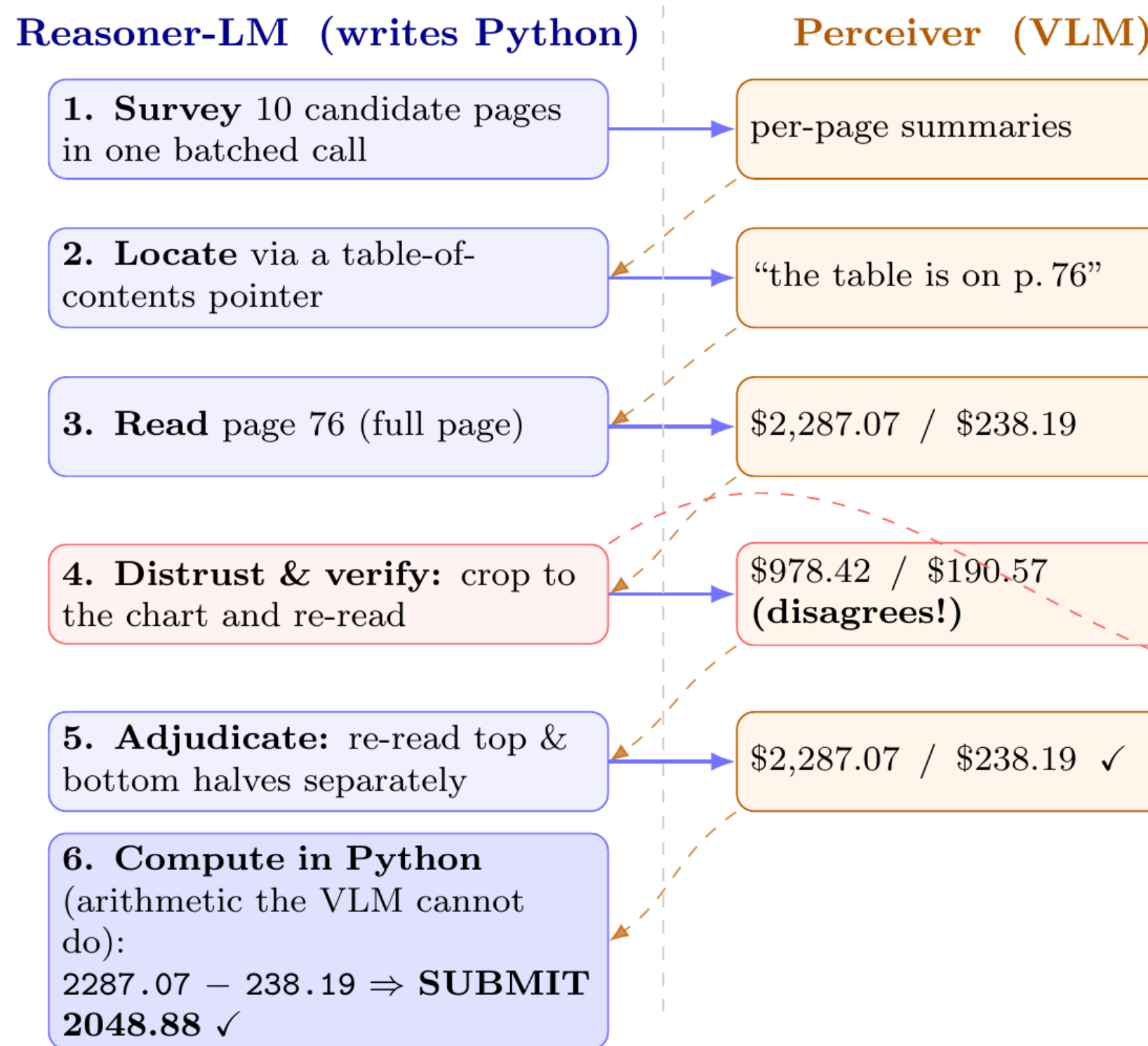
Fig. 1. Perceive-Reason-Code on a 181-page report. The reasoner-LM writes Python that calls the Perceiver (VLM) on regions it chooses: it surveys pages, locates the table, distrusts a full-page read, re-reads a tighter crop that disagrees, adjudicates, and computes the answer in Python — finding across pages and reading within one. The crop-verify catches a wrong number a single read would have submitted.
