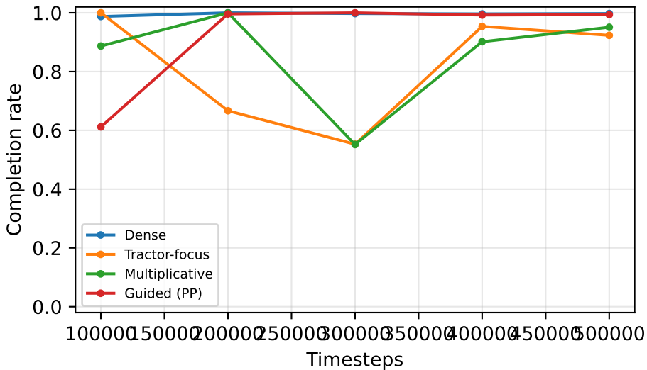
Forward (DQN)
