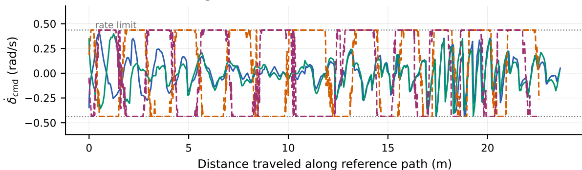
(c) Commanded steering rate
