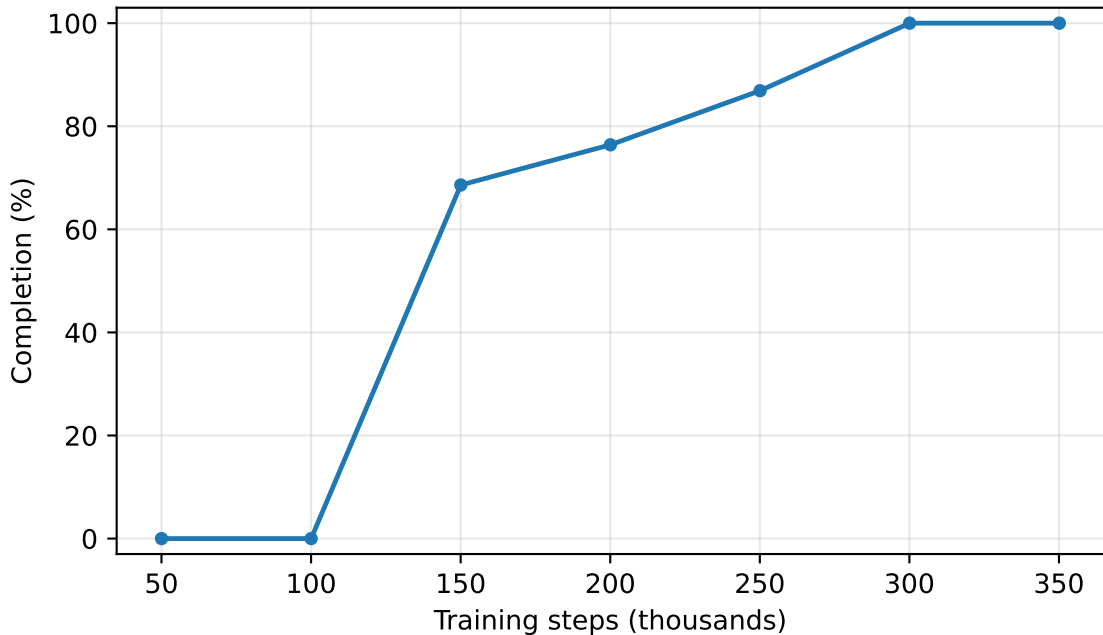
Geometry-encoder policy, forward lane-following (seed 0)
