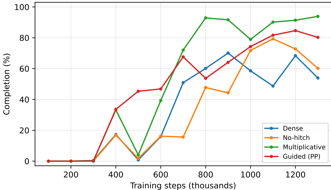
Reward ablation (TD3), reverse lane-following
