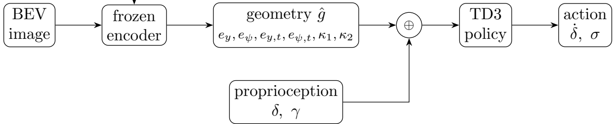
Figure 4.2: Geometry-distillation training. In Stage 1 a convolutional encoder is trained by supervised regression to predict the vehicle’s path geometry from the bird’s-eye-view image, using the simulator’s true state as a privileged teacher, and is then frozen. In Stage 2 the policy is trained from scratch with TD3 on the frozen geometry prediction concatenated with the steering and hitch angles supplied as proprioception.
