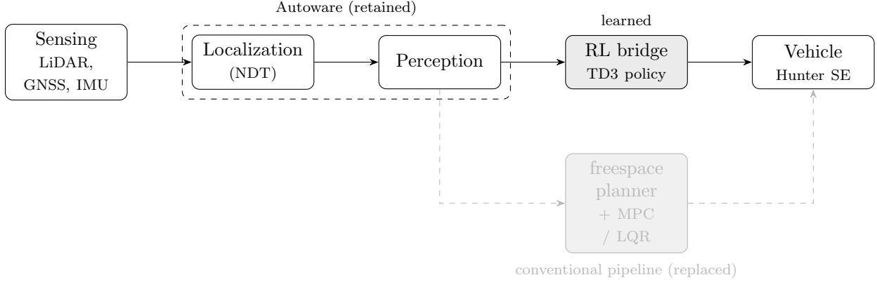
Figure 6.3: Deployment software stack. Autaware’s localization and perception are retained unchanged, while the planning and control layers (the conventional freespace planner and MPC/LQR tracker) are replaced by the learned RL bridge. The two control paths are mutually exclusive and selected at launch.
