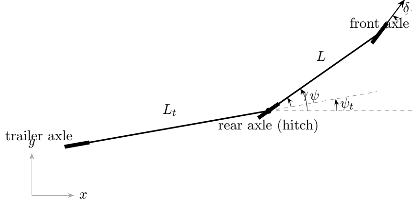
Figure 3.1: Tractor-trailer geometry. The tractor rear axle carries the hitch ( L_h \approx 0 ), from which the trailer of wheelbase L_t trails at articulation angle \gamma = \psi - \psi_t . The front wheel is steered by \delta relative to the tractor heading \psi , and L is the tractor wheelbase.
