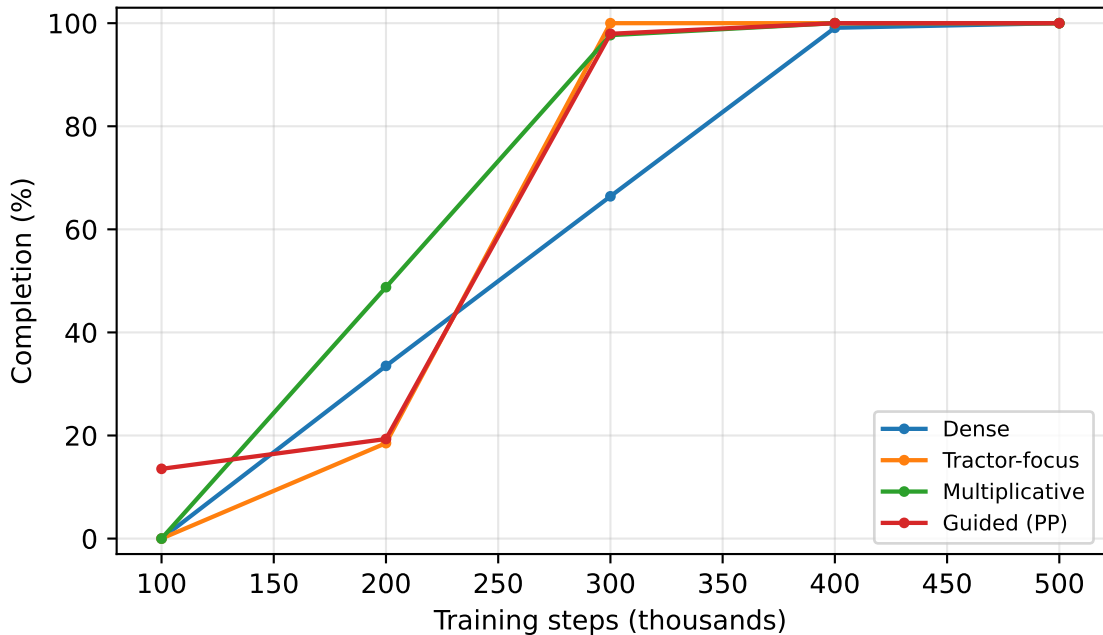
Reward ablation (TD3), forward lane-following
