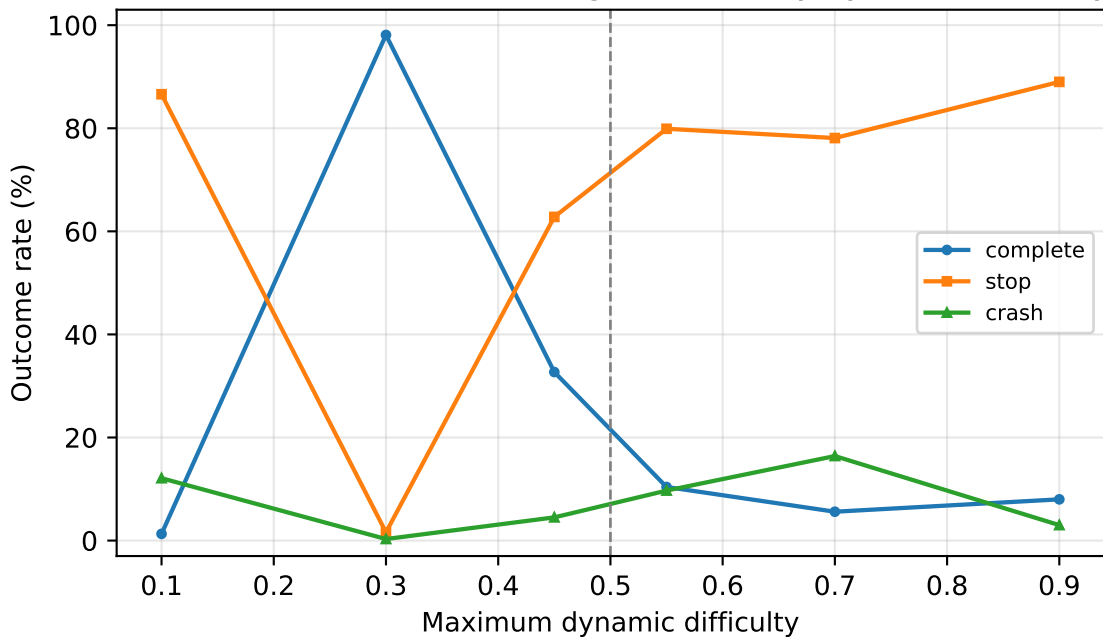
Reverse obstacle manoeuvring, outcome by dynamic difficulty
