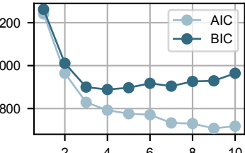
AIC and BIC for Different Numbers of Clusters
