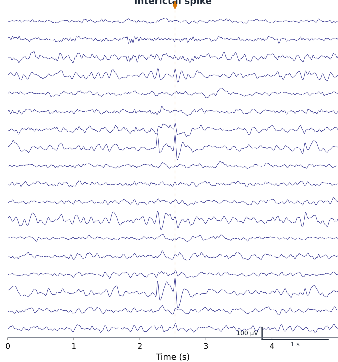
Interictal spike
