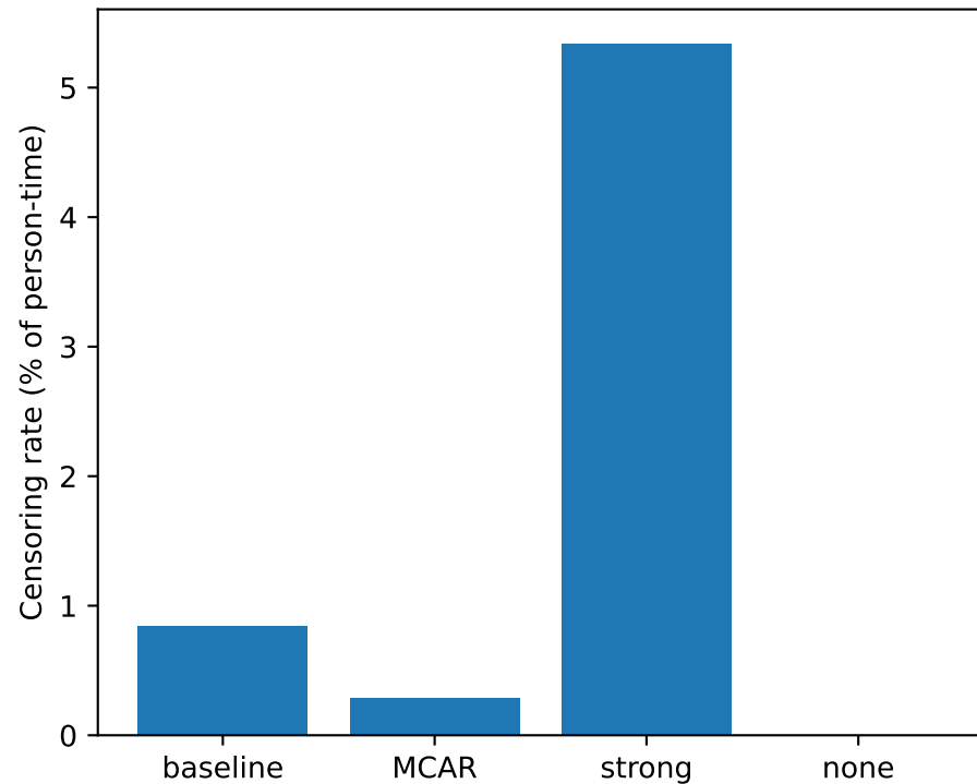
Censoring rate by regime
