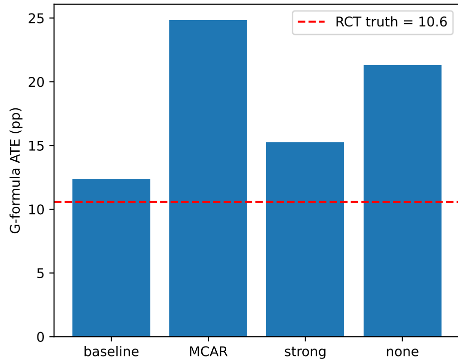
Recovered ATE across censoring regimes
