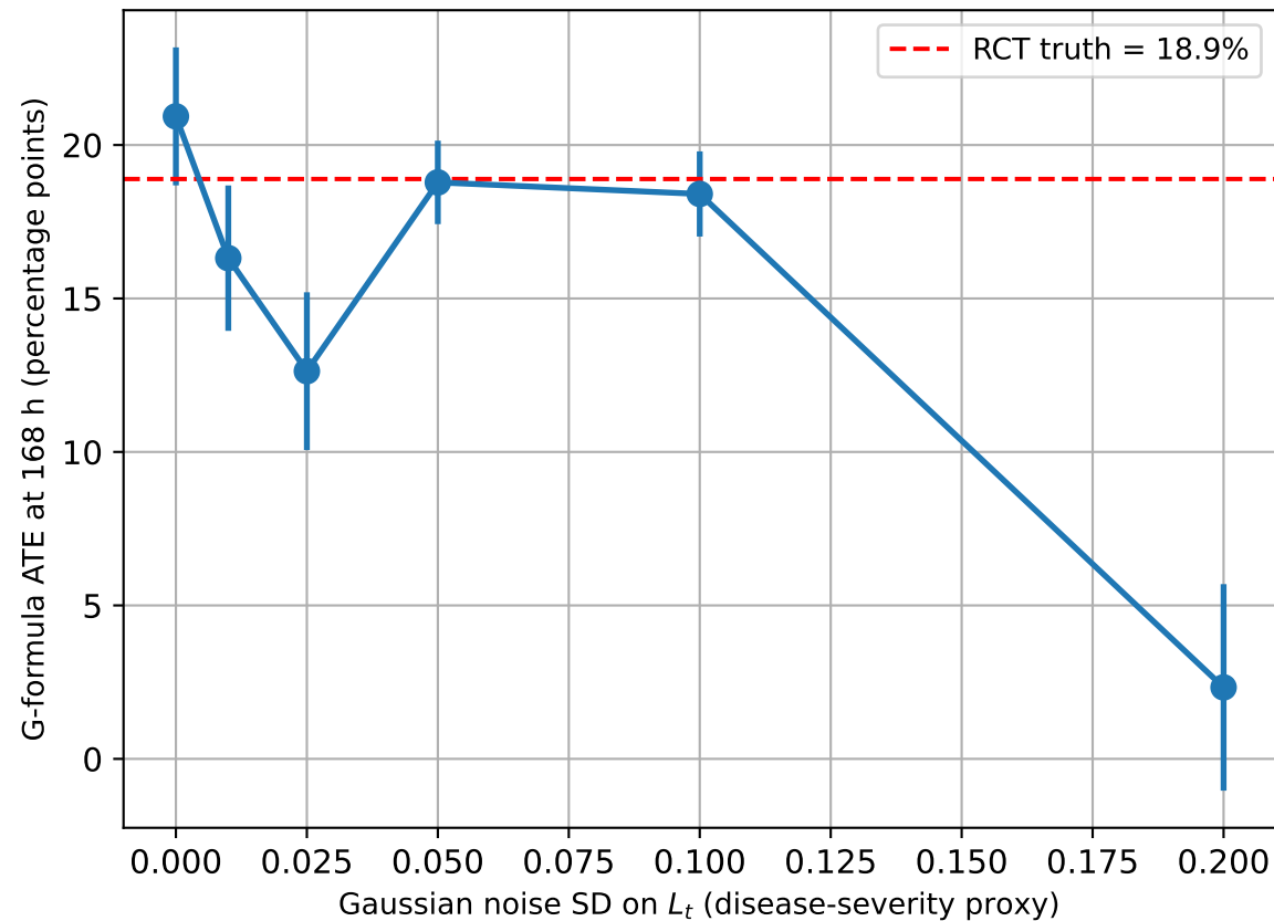
Measurement-error sensitivity of the CICADAS g-formula mean \pm SD across 3 seeds per \sigma
