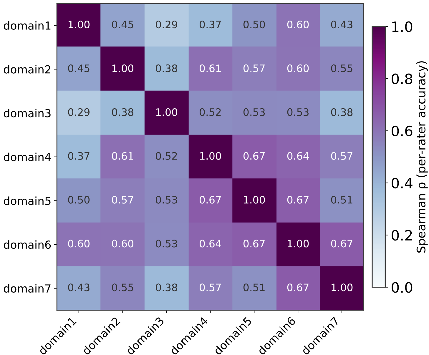
Cross-domain skill manifold — dual-contest cohort \rho(\text{domain1}, \text{domains2-7}) = 0.57 (n = 136, disattenuated 0.77)
