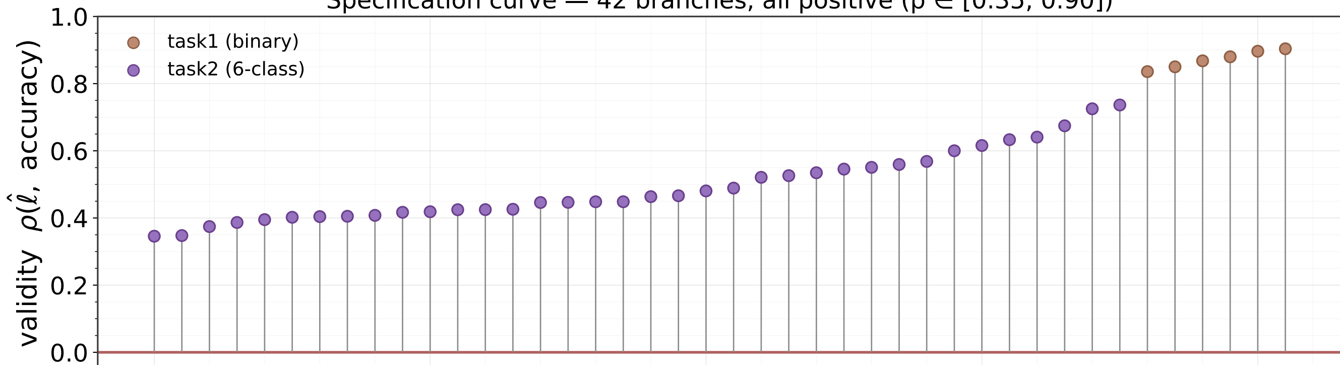
Specification curve — 42 branches, all positive ( \rho \in [0.35, 0.90] )
