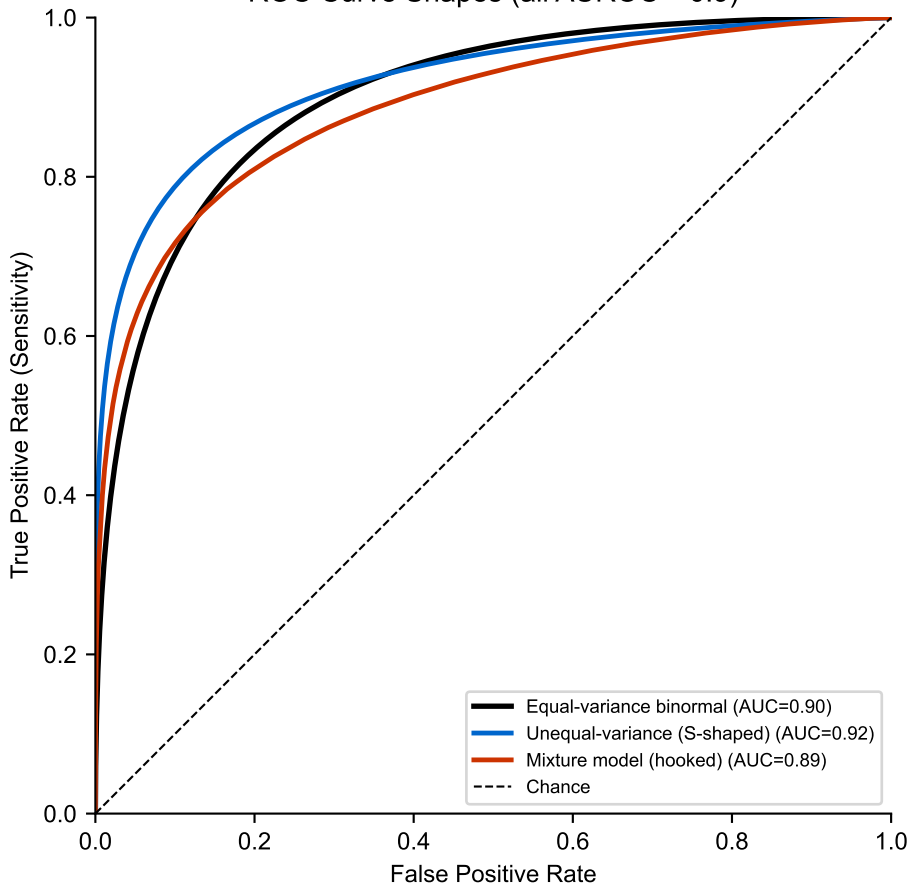
ROC Curve Shapes (all AUROC \approx 0.9 )
