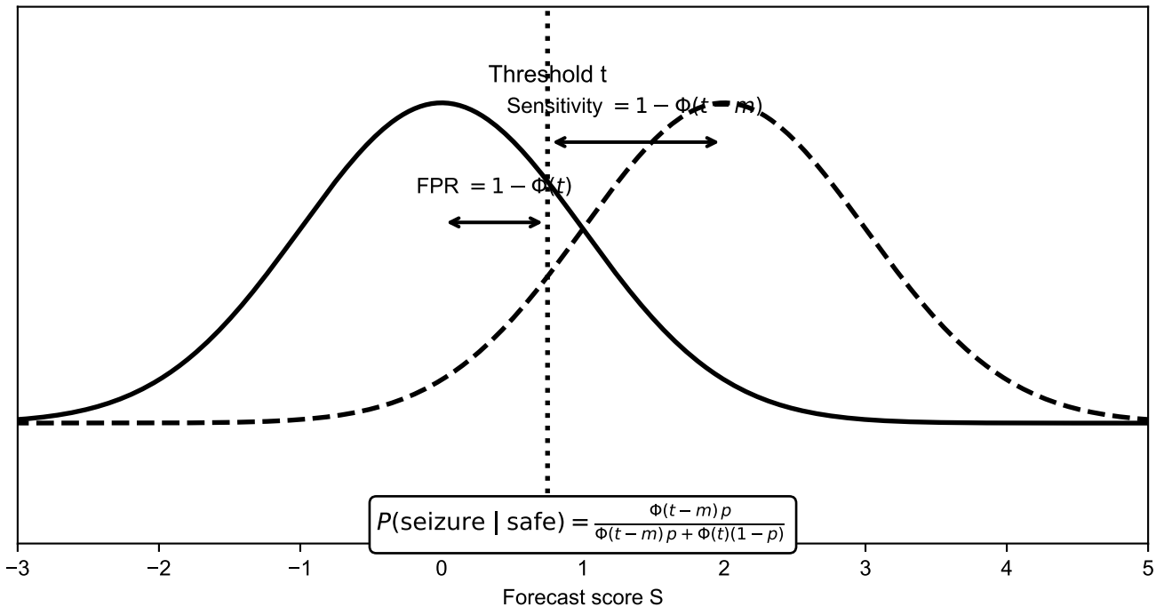
Schematic of Symmetric Binormal Forecast Model (Figure S0)
