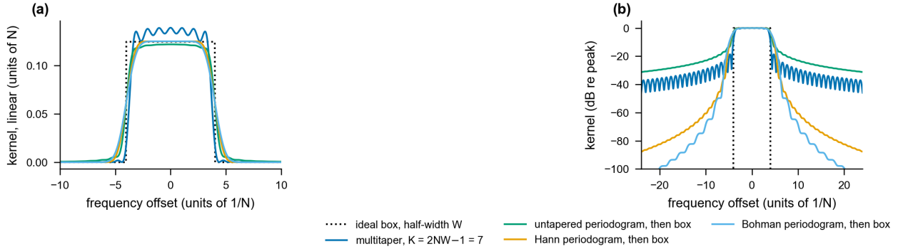
Figure S1: Kernels at the same design bandwidth ( N = 256 , W = 4/N ; Table II): (a) on a linear scale near the main lobe and (b) in dB relative to the peak. The ideal box; the K = 7 multitaper kernel ( \nu = 14.0 ); and the untapered ( \nu = 17.2 ), Hann ( \nu = 8.9 ) and Bohman ( \nu = 7.3 ) periodograms followed by the box. All main lobes have nearly the same width, and the skirts differ by 40 dB.
