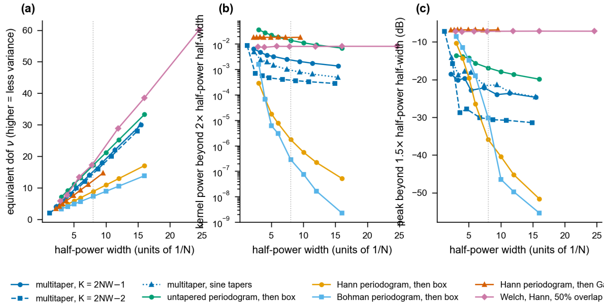
Figure S3: Variance, leakage and side-lobe level versus measured resolution for N = 256 . All curves are exact kernel and degrees-of-freedom computations, with no sampling variability. Each method's bandwidth parameter is swept and the quantities are plotted against the resulting half-power width, so methods are compared at equal resolution: multitaper with K = 2NW - 1 and 2NW - 2 Slepian tapers and with sine tapers; untapered, Hann and Bohman periodograms followed by a box; a Hann periodogram followed by a Gaussian; Welch's method with 50% overlap. (a) Equivalent degrees of freedom \nu (higher means less variance). (b) Kernel power beyond twice the half-power half-width. (c) The peak of the kernel beyond 1.5\times the half-power half-width. The Gaussian and Welch kernels have no flat top, so for them this quantity is the skirt of the main lobe and not a side lobe. The dotted line marks the 8/N width of Table II.
