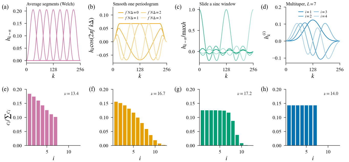
Figure 5: Three ways to build a bank of tapers from one window, and the reference bank ( N = 256 , R = 8/(N\Delta) ). (a–d) The bank as constructed, in one colour for each route, with lighter shades for later members of the bank in (b–d). (a) Welch’s method with Hann segments of length N/4 at 50% overlap: seven time-shifted copies of one window. (b) A periodogram tapered with a 25% cosine taper and smoothed with a parabola of half-power width R : frequency-shifted copies of one taper, four of a continuum. (c) A sinc window of bandwidth R slid across the record one sample at a time, four positions shown; in the limit of a long window this is exactly the untapered periodogram smoothed with a box, and exactly Thomson’s estimate with all N tapers weighted by \lambda_i . (d) Thomson’s estimate with L = 7 equally weighted Slepian tapers, the first four shown. (e–h) The eigen-weight ladder c_i of each, normalized to unit sum, whose flatness sets \nu = 2(\sum_i c_i)^2 / \sum_i c_i^2 by (15): \nu = 13.4, 16.7, 17.2 and 14.0 . The eigen-tapers of (c) are the Slepian sequences themselves. Fig. S4 adds the eigen-tapers and kernels.
