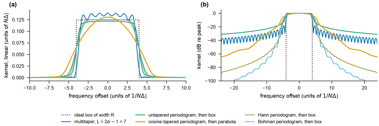
Figure S1: Kernels at the same design bandwidth ( N = 256 , R = 8/(N\Delta) ; Table II): (a) on a linear scale near the main lobe and (b) in dB relative to the peak. The ideal box; the L = 7 multitaper kernel ( \nu = 14.0 ); the periodogram after a 25% cosine taper followed by a parabola of the same half-power width ( \nu = 16.7 ), which is recipe (b’); and the untapered ( \nu = 17.2 ), Hann ( \nu = 8.9 ) and Bohman ( \nu = 7.3 ) periodograms followed by the box. All main lobes have nearly the same half-power width, and the skirts differ by 40 dB.
