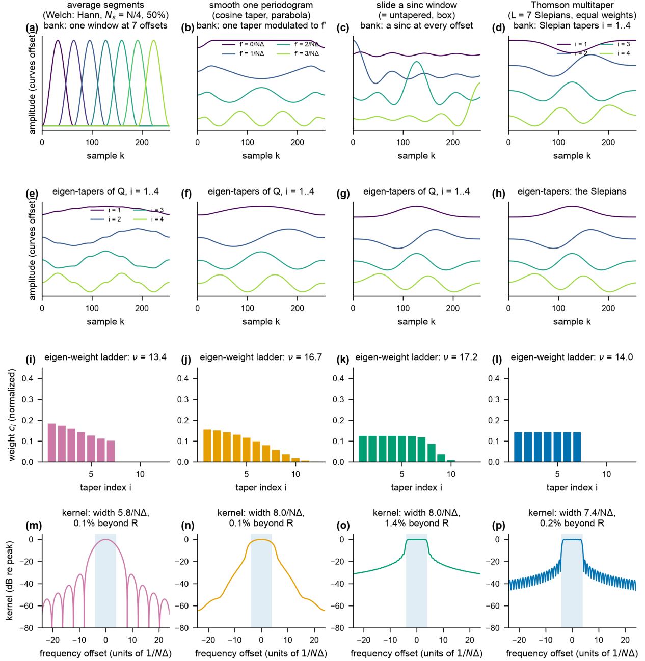
Figure S4: Fig. 5 in full. Columns as in Fig. 5; rows: the bank as constructed (a–d), the first four eigen-tapers of Q (e–h; for the sliding sinc they are the Slepian sequences, and for Thomson’s estimate, whose weights are equal, the Slepian are one of many orthonormal bases of the span), the eigen-weight ladder (i–l), and the kernel in dB relative to its peak with its half-power width and the fraction of its power beyond R (m–p; shading |f| \leq R/2 ).
