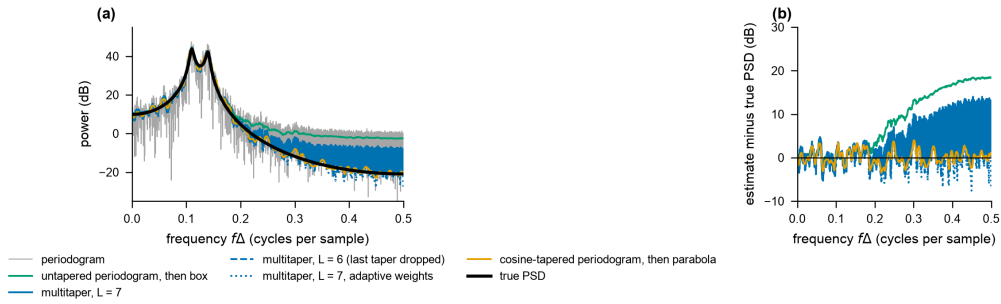
Figure S2: Dropping the leakiest taper. (a) One realization of the AR(4) process ( N = 1024 , R = 8/(N\Delta) ): the periodogram ( \nu = 2 , grey); the untapered periodogram smoothed with the box ( \nu = 17.2 , green); the equal-weight multitaper estimate with L = 7 ( \nu = 14 , solid blue) and with L = 6 ( \nu = 12 , dashed blue), and the adaptively weighted estimate with L = 7 (dotted blue); the cosine-tapered periodogram smoothed with a parabola of half-power width R ( \nu = 16.7 , orange); and the true PSD (black). (b) Each smoothed estimate minus the true PSD: the untapered box floors 20 dB high, L = 7 floors 10 dB high, dropping the seventh taper halves that, and the adaptive weights and the smoothed periodogram track the truth.
