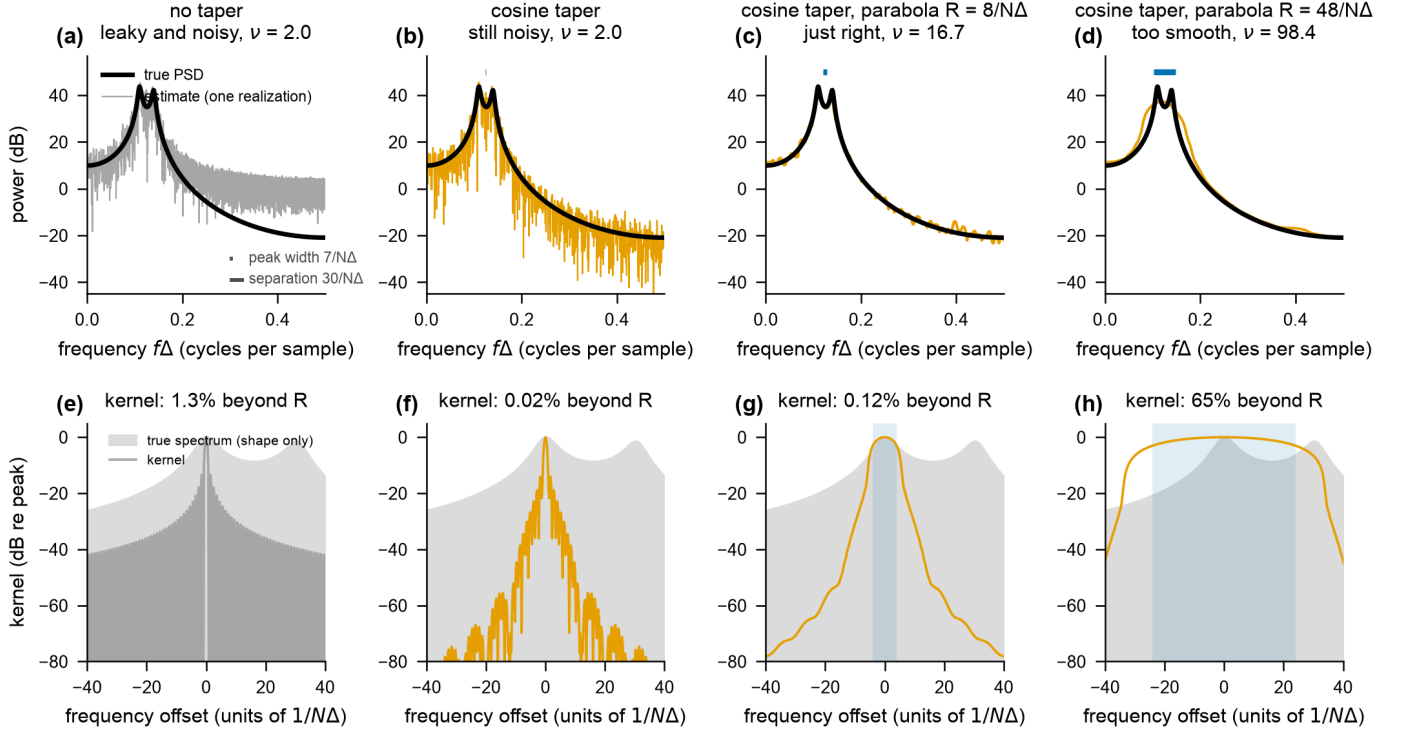
Fig. 2. Every estimator is the true spectrum blurred by a kernel, plus noise. (a–d) One realization ( N = 1024 ) of an autoregressive process whose PSD (black) has two peaks 7/(N\Delta) wide at half power and 30/(N\Delta) apart on a background spanning 65 dB, estimated by the periodogram (a), the periodogram of the record after a 25% cosine taper (b), the same smoothed with a parabola whose half-power width R = 8/(N\Delta) is that of a peak (c), and smoothed with R = 48/(N\Delta) , which exceeds the separation of the peaks (d). The short blue bar above the peaks is the half-power width of each estimator's kernel, and the grey bars in (a) mark the peak width and separation. The equivalent degrees of freedom are denoted \nu . (e–h) Each estimator's expected-value kernel in dB relative to its peak, drawn over the true spectrum around its peaks (grey, showing its shape only). Blue shading marks |f| \leq R/2 . The panel titles give the fraction of the kernel's power outside |f| \leq R , which is our measure of broadband leakage. The skirts of the Fejér kernel fall slowly, so power leaks from the peaks into the region 40 dB below them (a, e). The cosine taper lowers the skirts by 22 dB at 16/(N\Delta) and by 39 dB at 40/(N\Delta) , and widens the main lobe by 15% (f). A kernel as wide as a peak is just right (g), and a wider kernel merges the peaks (h).
