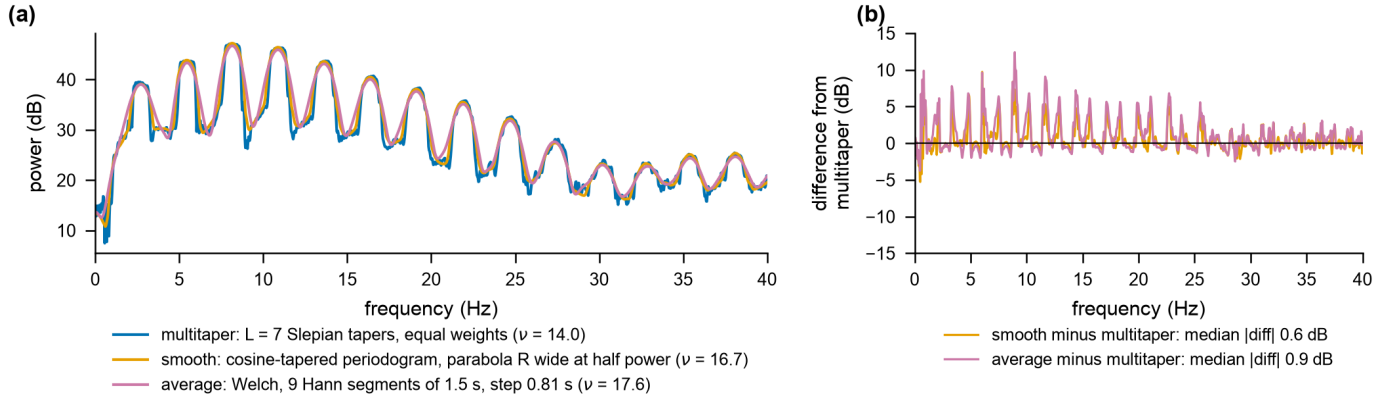
Fig. 7. The estimators used in practice agree to within their own noise. (a) The EEG epoch of Fig. 1 estimated by Thomson's method with L = 7 tapers ( \nu = 14 , blue); by a cosine-tapered periodogram smoothed with a parabola of half-power width R ( \nu = 16.7 , orange); and by Welch's method with nine Hann segments of 1.5 s stepped by 0.81 s ( \nu = 17.6 , purple). Their half-power widths are 0.91, 1.03 and 0.97 Hz. (b) Differences from the multitaper estimate: median absolute difference 0.6 dB (smoothed) and 0.9 dB (averaged), 95th percentiles 4.2 and 5.9 dB. The medians are smaller than the estimators' own noise ( 4.3\sqrt{2/\nu} gives 1.6, 1.5 and 1.5 dB). The largest differences are in the valleys between harmonics, which the seventh Slepian taper's side lobes fill in.
