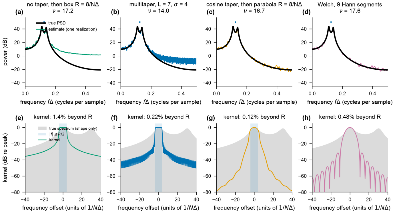
Fig. 6. The estimators used in practice, applied to the record of Fig. 2 ( N = 1024 , R = 8/(N\Delta) ; one realization). (a–d) The untapered periodogram smoothed with a box, which is the exact estimate (16) (green); Thomson's estimate with L = 7 tapers (blue); a cosine-tapered periodogram smoothed with a parabola of the same half-power width (orange); and Welch's method with nine Hann segments of 192 samples stepped by 104, chosen for approximately the same half-power width (purple; the four widths are 8.2, 7.2, 8.2 and 7.8/(N\Delta) ). This realization has more leakage than is typical. Its median absolute errors over the band are 11.6, 4.6, 0.9 and 0.8 dB, and the values over 300 realizations are 5.3, 2.3, 1.0 and 1.0 dB (Table I). (e–h) The kernels, as in Fig. 2. The untapered box (e) inherits the Fejér tails, and its estimate levels off 20 dB above the true spectrum. The seventh Slepian taper puts the skirt of the multitaper kernel at -22 dB (f), and that estimate levels off 10 dB above the true spectrum. The kernel of the cosine-tapered parabola (g) has no side lobes and falls below -38 dB beyond 1.5R . Welch's kernel (h) has no flat top, and its side lobes are spaced at the scale of the peaks.
