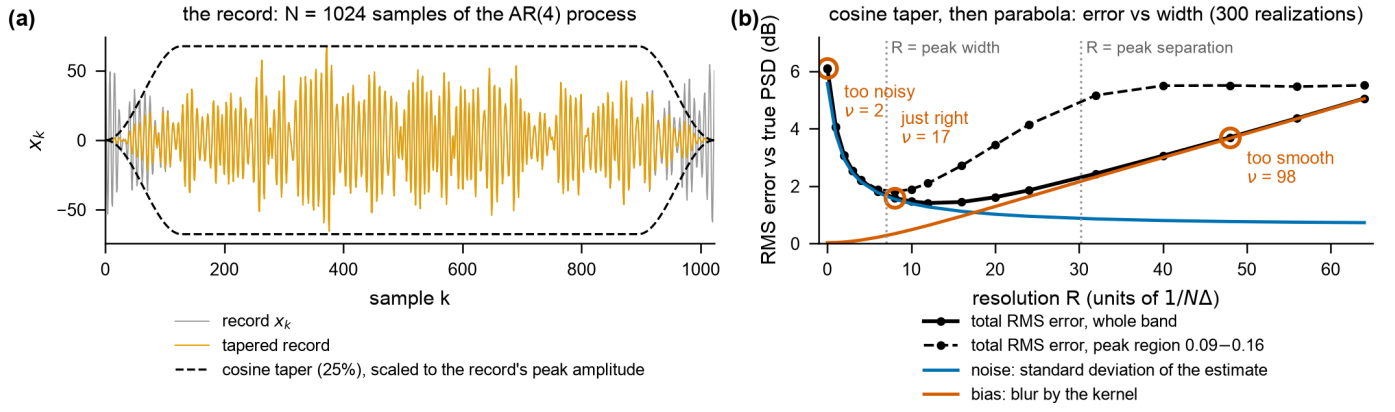
Fig. 3. Choosing the bandwidth. (a) The record of Fig. 2: N = 1024 samples of the AR(4) process (grey), the 25% cosine taper scaled to the record's peak amplitude (dashed), and the tapered record (orange). (b) Root-mean-square error over frequency, in dB, of the cosine-tapered periodogram smoothed with a parabola of half-power width R , against the true PSD as R varies, averaged over 300 independent realizations; no error bars are shown because the curves are ensemble averages. Noise (the standard deviation of the estimate, blue) falls with R , blur (the bias of the kernel, orange) grows, and their total (black) has a broad minimum that sits at smaller R when only the peak region, 0.09 \leq f\Delta \leq 0.16 , is scored (dashed). The circled points are panels (b), (c) and (d) of Fig. 2.
