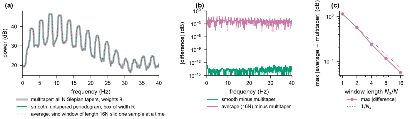
Fig. 1. Three routes to one spectrum. (a) Power spectral density (PSD) of eight seconds of one channel of de-identified scalp EEG at 128 Hz from the authors' archive ( N = 1024 ; one epoch), design resolution R = 8/(N\Delta) = 1 Hz ( \alpha = 4 ), by three routes: the multitaper estimate with all N Slepian tapers weighted by their eigenvalues \lambda_i (thick grey); the untapered periodogram smoothed with a box of width R (green); and the average of periodograms of a sinc window of bandwidth R and length 16N slid across the record one sample at a time (dashed purple). (b) Absolute differences from the multitaper estimate on a logarithmic scale: the smoothed periodogram agrees to 3 \times 10^{-13} dB, the sliding-window average to 0.06 dB. (c) The maximum difference of the sliding-window average versus window length N_s , with a 1/N_s guide line. The multitaper estimate here has \nu = 17 equivalent degrees of freedom, as defined in Section II-B.
