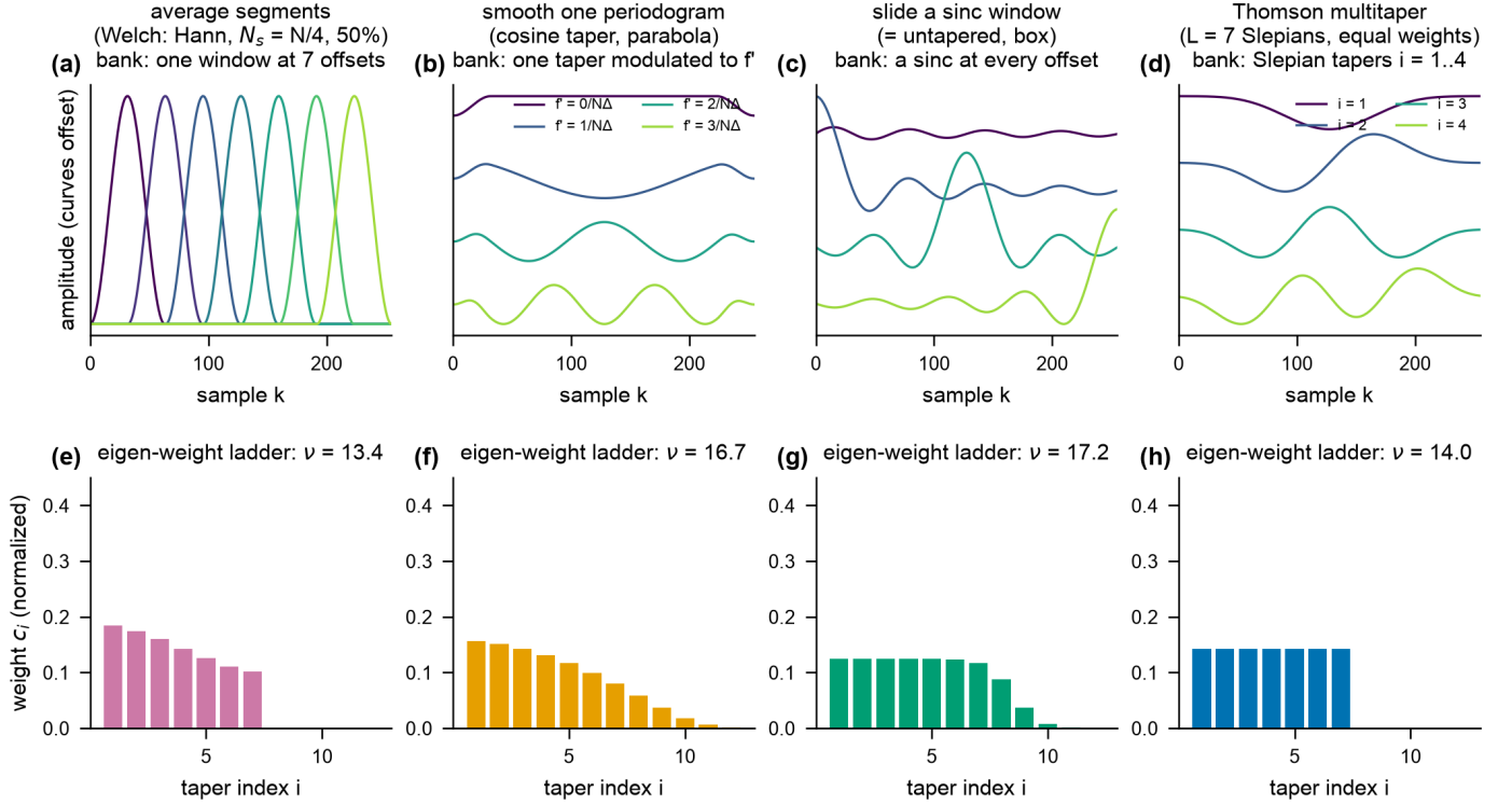
Fig. 5. Three ways to build a bank of tapers from one window, and the reference bank. N = 256 , R = 8/(N\Delta) . (a–d) The bank as constructed: (a) Welch’s method with Hann segments of length N/4 at 50% overlap (seven time-shifted copies of one window); (b) a periodogram tapered with a 25% cosine taper and smoothed with a parabola of half-power width R (frequency-shifted copies of one taper, four of a continuum shown); (c) a sinc window of bandwidth R slid across the record one sample at a time, which in the limit of a long window is exactly the untapered periodogram smoothed with a box and exactly Thomson’s estimate with all N tapers weighted by \lambda_i ; (d) Thomson’s estimate with L = 7 equally weighted Slepian tapers. (e–h) The eigen-weight ladder c_i of each, normalized to unit sum, whose flatness sets \nu = 2(\sum_i c_i)^2 / \sum_i c_i^2 by (15). The eigen-tapers of (c) are the Slepian sequences themselves. Fig. S4 adds the eigen-tapers and kernels.
