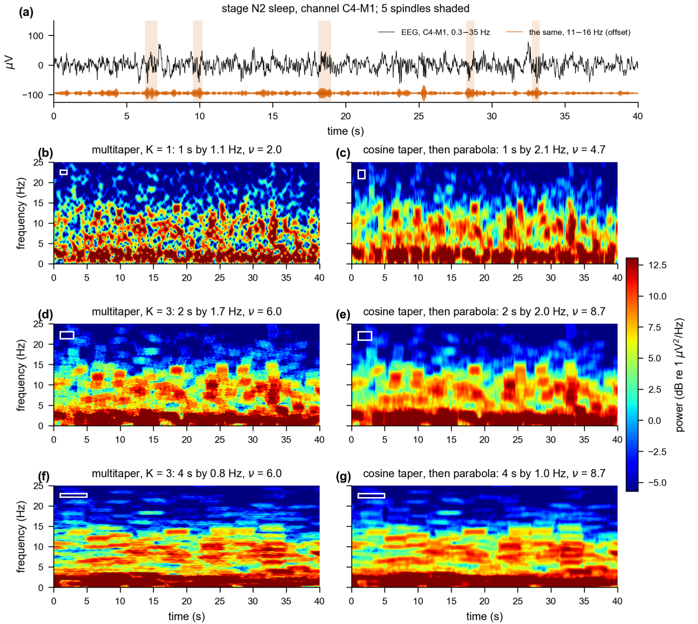
Fig. 9. Sleep spindles at three resolutions. (a) Forty seconds of stage N2 sleep, channel C4-M1, filtered between 0.3 and 35 Hz (black) and between 11 and 16 Hz (orange, offset), with five spindles shaded. (b–g) Spectrograms from windows of 1 s (b, c), 2 s (d, e) and 4 s (f, g) stepped by 0.1 s, by the multitaper estimate with L = 2\alpha - 1 tapers (left) and by a cosine-tapered periodogram smoothed with a parabola (right), on one colour scale. The titles give the window length, the half-power width of the kernel and \nu . The white box has these dimensions, so it shows the resolution of the panel, and twice its area is approximately \nu . Short windows keep the spindles brief and blur them in frequency, and long windows do the opposite.
