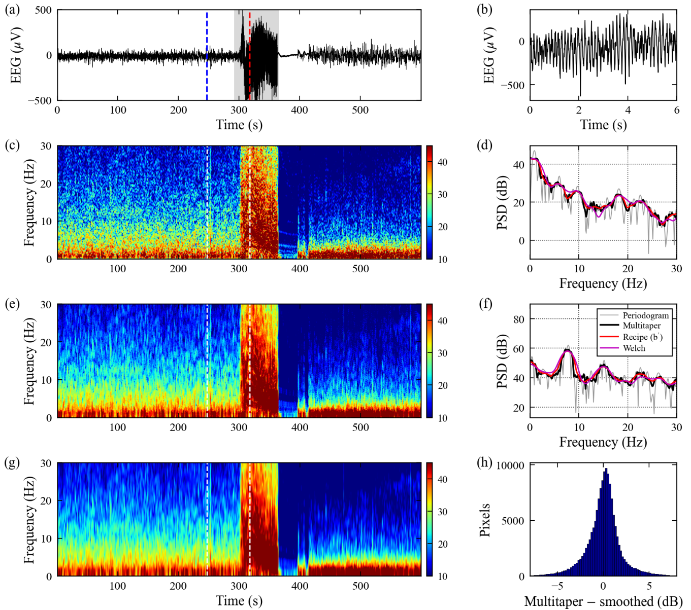
Figure 8: Three estimators of a seizure. (a) Ten minutes of de-identified scalp EEG at 200 Hz (ELROND seizure-annotation set), channel C4 against the common average, displayed between \pm 500 \mu V ; the seizure is shaded and the dashed lines mark the instants used in (d) and (f). (b) Six seconds of the ictal rhythm from t = 318 s. (c, e, g) Spectrograms from 599 windows of 2 s stepped by 1 s: the periodogram after a 25% cosine taper ( \nu = 2 ), the multitaper estimate with \alpha = 2 , L = 3 ( \nu = 6 ), and the same periodogram smoothed with a parabola 2 Hz wide at half power ( \nu = 8.7 ), on one colour scale of 10 to 45 dB. (d, f) Spectra at the pre-ictal and ictal instants by all three, plus Welch’s method with 0.7-second Hann segments ( \nu = 7.7 ). (h) Distribution over all pixels of the difference between (e) and (g). The channel is the one with the largest ictal rise in 2 to 20 Hz power.
