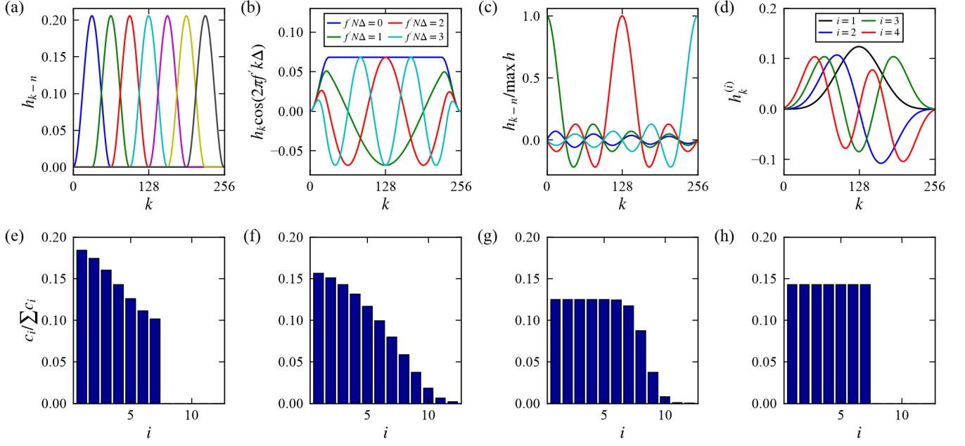
Figure 5: Three ways to build a bank of tapers from one window, and the reference bank ( N = 256 , R = 8/(N\Delta) ). (a–d) The bank as constructed. (a) Welch’s method with Hann segments of length N/4 at 50% overlap: seven time-shifted copies of one window. (b) A periodogram tapered with a 25% cosine taper and smoothed with a parabola of half-power width R : frequency-shifted copies of one taper, four of a continuum. (c) A sinc window of bandwidth R slid across the record one sample at a time, four positions shown; in the limit of a long window this is exactly the untapered periodogram smoothed with a box, and exactly Thomson’s estimate with all N tapers weighted by \lambda_i . (d) Thomson’s estimate with L = 7 equally weighted Slepian tapers, the first four shown. (e–h) The eigen-weight ladder c_i of each, normalized to unit sum, whose flatness sets \nu = 2(\sum_i c_i)^2 / \sum_i c_i^2 by (15): \nu = 13.4, 16.7, 17.2 and 14.0 . The eigen-tapers of (c) are the Slepian sequences themselves. Fig. S4 adds the eigen-tapers and kernels.
