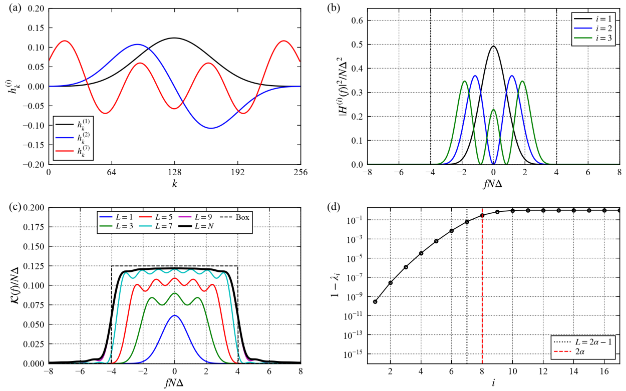
Figure 4: Why the multitaper kernel is a box ( N = 256 , R = 8/(N\Delta) ). (a) The first (black), second (blue) and seventh (red) Slepian tapers. (b) The kernels |H^{(i)}(f)|^2/\Delta of the first three, each filling the gaps left by the previous ones within the band |f| \leq R/2 (dotted lines). (c) The running sum \sum_{i \leq L} \lambda_i |H^{(i)}(f)|^2 / 2\alpha\Delta as tapers are added. With all N tapers it is exactly the box of width R convolved with Fejér’s kernel, which is the identity (16) in kernel form and cannot be distinguished from the box itself (dashed) at this scale. With the usual L = 2\alpha - 1 = 7 it is the box with rounded shoulders and small ripple. (d) The concentration ladder: the fraction 1 - \lambda_i of each taper’s energy outside the band. Tapers beyond the 2\alpha th carry only leakage.
