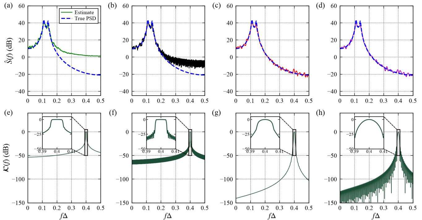
Figure 6: The estimators used in practice, applied to the record of Fig. 2 ( N = 1024 , R = 8/(N\Delta) ; one realization; true PSD blue, dashed). (a) The untapered periodogram smoothed with a box, which is the exact estimate (16) ( \nu = 17.2 ). (b) Thomson's estimate with L = 7 tapers ( \nu = 14.0 ). (c) A cosine-tapered periodogram smoothed with a parabola of the same half-power width ( \nu = 16.7 ). (d) Welch's method with nine Hann segments of 192 samples stepped by 104, chosen for about the same half-power width ( \nu = 17.6 ). The four half-power widths are 8.2, 7.2, 8.2 and 7.8/( N\Delta ). This realization has more leakage than is typical. Its median absolute errors over the band are 11.6, 4.6, 0.9 and 0.8 dB, and the values over 300 realizations are 5.3, 2.3, 1.0 and 1.0 dB (Table 1). (e–h) The kernels, as in Fig. 2, with 1.4%, 0.22%, 0.12% and 0.48% of their power outside |f| \leq R . The untapered box (e) inherits the Fejér tails, and its estimate levels off 20 dB above the true spectrum. The seventh Slepian taper puts the skirt of the multitaper kernel at -22 dB (f), and that estimate levels off 10 dB above the true spectrum. The kernel of the cosine-tapered parabola (g) has no side lobes and falls below -38 dB beyond 1.5R . Welch's kernel (h) has no flat top, and its side lobes are spaced at the scale of the peaks.
