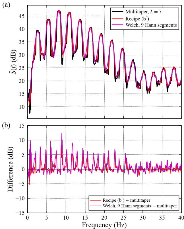
Figure 7: The estimators used in practice agree to within their own noise. (a) The EEG epoch of Fig. 1 estimated by Thomson’s method with L = 7 tapers ( \nu = 14 , black), by a cosine-tapered periodogram smoothed with a parabola of half-power width R , recipe (b') ( \nu = 16.7 , red), and by Welch’s method with nine Hann segments of 1.5 s stepped by 0.81 s ( \nu = 17.6 , magenta). Their half-power widths are 0.91, 1.03 and 0.97 Hz. (b) Differences from the multitaper estimate: median absolute difference 0.6 dB (smoothed) and 0.9 dB (averaged), 95th percentiles 4.2 and 5.9 dB. The medians are smaller than the estimators’ own noise ( 4.3\sqrt{2/\nu} gives 1.6, 1.5 and 1.5 dB). The largest differences are in the valleys between harmonics, which the side lobes of the seventh Slepian taper fill in.
