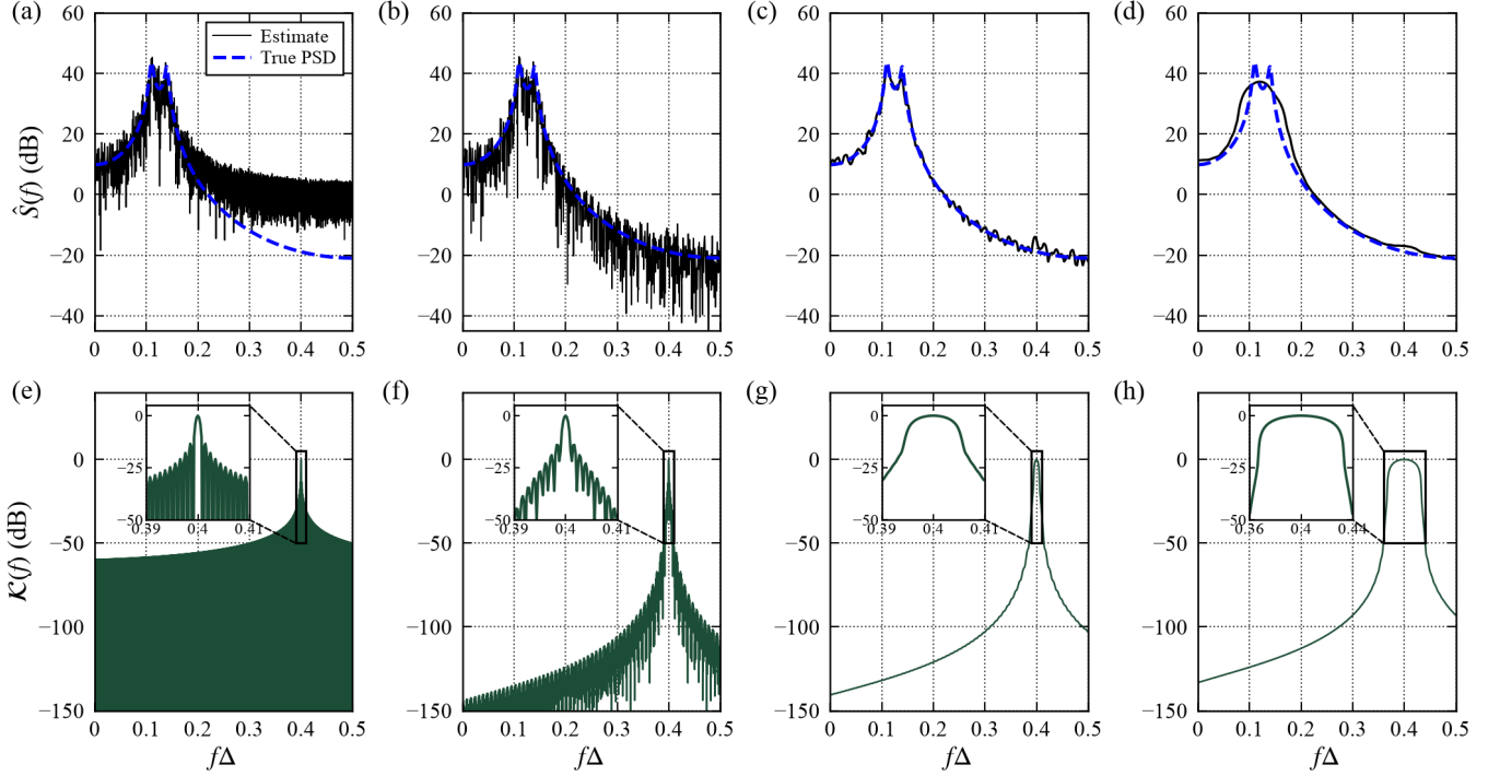
Figure 2: Every estimator is the true spectrum blurred by a kernel, plus noise. One realization ( N = 1024 ) of an autoregressive process whose PSD (blue, dashed) has two peaks 7/(N\Delta) wide at half power and 30/(N\Delta) apart on a background spanning 65 dB. (a) Periodogram estimate. (b) Periodogram of the record after a 25% cosine taper. (c) The same, smoothed with a parabola whose half-power width R = 8/(N\Delta) is that of a peak. (d) Smoothed with R = 48/(N\Delta) , which exceeds the separation of the peaks. The equivalent degrees of freedom are \nu = 2, 2, 16.7 and 98.4 . (e–h) The expected-value kernel of each estimator in dB relative to its peak, centered at f\Delta = 0.4 . The zoomed-in view of the main lobe is shown on the top left. The half-power widths are 0.8, 1.2, 8.2 and 47.8/(N\Delta) , and 1.3\%, 0.02\%, 0.12\% and 65\% of the kernel’s power lies outside |f| \leq 8/(N\Delta) , our measure of broadband leakage. The skirts of the Fejér kernel fall slowly, so power leaks from the peaks into the region 40 dB below them (a, e). The cosine taper lowers the skirts by 22 dB at 16/(N\Delta) and by 39 dB at 40/(N\Delta) , and widens the main lobe by 15% (f). A kernel as wide as a peak is just right (g), and a wider kernel merges the peaks (h).
