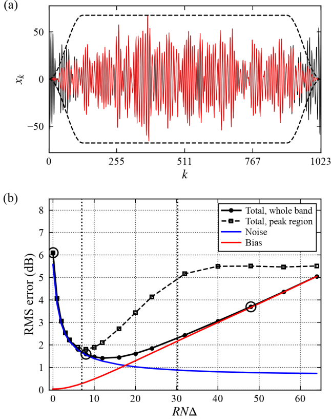
Figure 3: Choosing the resolution. (a) The record of Fig. 2, N = 1024 samples of the AR(4) process (black), the 25% cosine taper scaled to the record’s peak amplitude (dashed), and the tapered record (red). (b) Root-mean-square error over frequency, in dB, of the cosine-tapered periodogram smoothed with a parabola of half-power width R , against the true PSD, averaged over 300 independent realizations; the curves are ensemble averages and carry no error bars. The noise (the standard deviation of the estimate, blue) falls with R , the bias (blur by the kernel, red) grows, and their total over the whole band (solid black) has a broad minimum, which sits at smaller R when only the peak region, 0.09 \leq f\Delta \leq 0.16 , is scored (dashed). The circled points are panels (b), (c) and (d) of Fig. 2, and the dotted lines mark R equal to the width of a peak and to the separation of the peaks.
