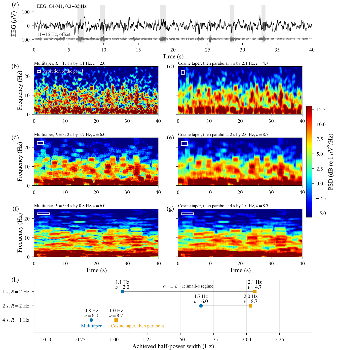
Figure 9: Sleep spindles at three resolutions. (a) Forty seconds of stage N2 sleep, channel C4-M1, filtered between 0.3 and 35 Hz (black) and between 11 and 16 Hz (grey, offset), with five spindles shaded. (b–g) Spectrograms from windows of 1 s (b, c), 2 s (d, e) and 4 s (f, g) stepped by 0.1 s, by the multitaper estimate with L = 2\alpha - 1 tapers, at least one (left), and by a cosine-tapered periodogram smoothed with a parabola (right), on one colour scale. The white box is the window length by the achieved half-power width, so it shows the resolution of the panel, and twice its area is approximately \nu . (h) Achieved half-power widths and equivalent degrees of freedom for multitaper (blue circles) and smoothing (orange squares) at each setting. At 1 s, \alpha = 1 and the practical multitaper rule gives L = 1 , so its achieved width is 1.1 Hz against 2.1 Hz for smoothing; at \alpha = 2 the widths are much closer. Short windows keep the spindles brief and blur them in frequency, and long windows do the opposite.
