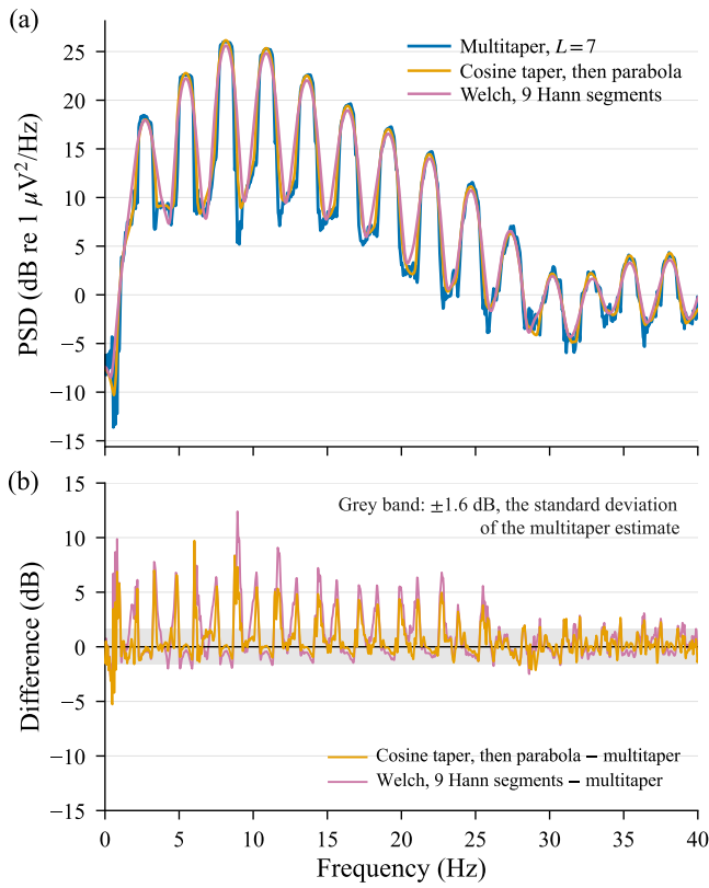
Figure 7: The estimators used in practice agree to within their own noise. (a) The EEG epoch of Fig. 1, in dB relative to 1 \mu\text{V}^2/\text{Hz} , estimated by Thomson’s method with L = 7 tapers ( \nu = 14 , blue), by a cosine-tapered periodogram smoothed with a parabola of half-power width R , recipe (b’) ( \nu = 16.7 , orange), and by Welch’s method with nine Hann segments of 1.5 s stepped by 0.81 s ( \nu = 17.6 , pink). Their half-power widths are 0.91, 1.03 and 0.97 Hz. (b) Differences from the multitaper estimate over the 1281 frequencies shown: median absolute difference 0.6 dB (smoothed) and 0.9 dB (averaged), 95th percentiles 4.2 and 5.9 dB. The medians are smaller than the estimators’ own noise (the standard deviation in dB of an estimate with \nu degrees of freedom, 4.3\sqrt{2/\nu} , gives 1.6, 1.5 and 1.5 dB; the grey band is \pm 1.6 dB). The largest differences are in the valleys between harmonics, which the side lobes of the seventh Slepian taper fill in.
