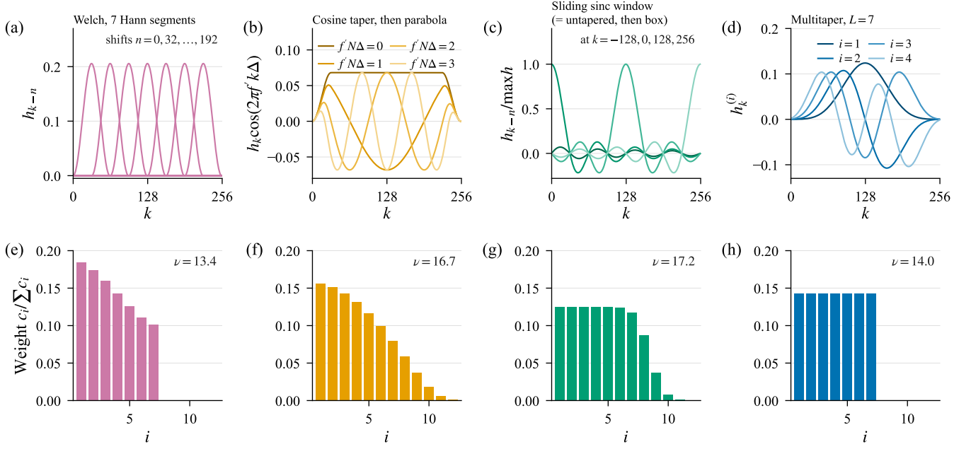
Figure 5: Three ways to build a bank of tapers from one window, and the reference bank ( N = 256 , R = 8/(N\Delta) , \alpha = 4 ). Every curve and weight is computed exactly. (a–d) The bank as constructed, in one colour for each route, with lighter shades for later members of the bank in (b–d). (a) Welch’s method with Hann segments of length N/4 at 50% overlap: seven time-shifted copies of one window. (b) A periodogram tapered with a 25% cosine taper and smoothed with a parabola of half-power width R : frequency-shifted copies of one taper, four of a continuum. (c) A sinc window of bandwidth R slid across the record one sample at a time, four positions shown; in the limit of a long window this is exactly the untapered periodogram smoothed with a box, and exactly Thomson’s estimate with all N tapers weighted by \lambda_i . (d) Thomson’s estimate with L = 7 equally weighted Slepian tapers, the first four shown. (e–h) The eigen-weight ladder c_i of each, normalized to unit sum, whose flatness sets \nu = 2(\sum_i c_i)^2 / \sum_i c_i^2 by (15): \nu = 13.4, 16.7, 17.2 and 14.0 . The eigen-tapers of (c) are the Slepian sequences themselves. Fig. S1 adds the eigen-tapers and kernels.
