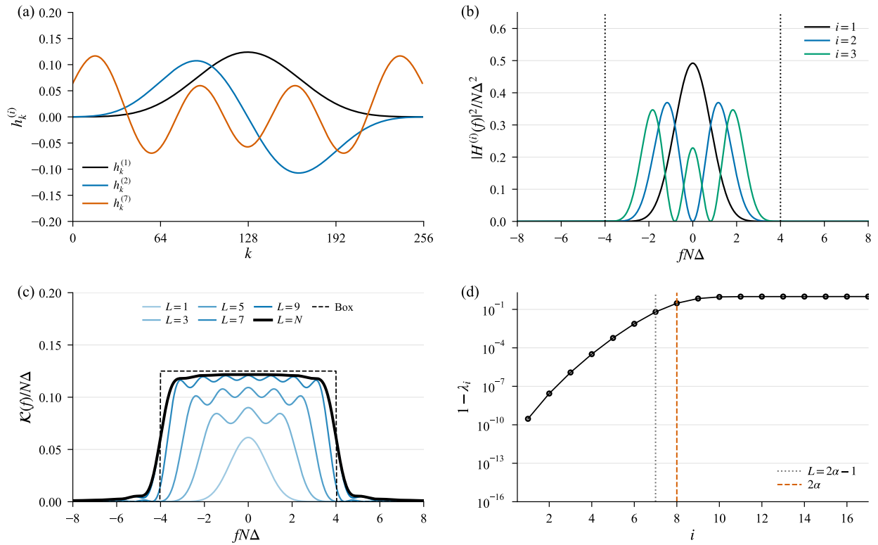
Figure 4: Why the multitaper kernel is a box ( N = 256 , R = 8/(N\Delta) ). (a) The first, second and seventh Slepian tapers. (b) The kernels |H^{(i)}(f)|^2/\Delta of the first three, each filling the gaps left by the previous ones within the band |f| \leq R/2 (dotted lines). (c) The running sum \sum_{i \leq L} \lambda_i |H^{(i)}(f)|^2/2\alpha\Delta as tapers are added, darker for larger L . With all N tapers it is exactly the box of width R convolved with Fejér’s kernel, which is the identity (16) in kernel form and cannot be distinguished from the box itself (dashed) at this scale. With the usual L = 2\alpha - 1 = 7 it is the box with rounded shoulders and small ripple. (d) The concentration ladder: the fraction 1 - \lambda_i of each taper’s energy outside the band. Tapers beyond the 2\alpha th carry only leakage.
