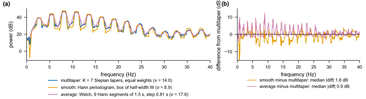
Figure 7: The estimators used in practice agree to within their own noise. (a) The EEG epoch of Fig. 1 estimated by Thomson’s method with K = 7 tapers ( \nu = 14 , blue); by a Hann-tapered periodogram smoothed with the same box ( \nu = 8.9 , orange); and by Welch’s method with nine Hann segments of 1.5 s stepped by 0.81 s ( \nu = 17.6 , purple). Their half-power widths are 0.91, 1.03 and 0.97 Hz. (b) Differences from the multitaper estimate: median absolute difference 1.6 dB (smoothed) and 0.9 dB (averaged), 95th percentiles 4.9 and 5.9 dB, which is the size of the estimators’ own noise ( 4.3\sqrt{2/\nu} gives 1.6, 2.1 and 1.5 dB). The largest differences are in the valleys between harmonics, which the seventh Slepian taper’s side lobes fill in.
