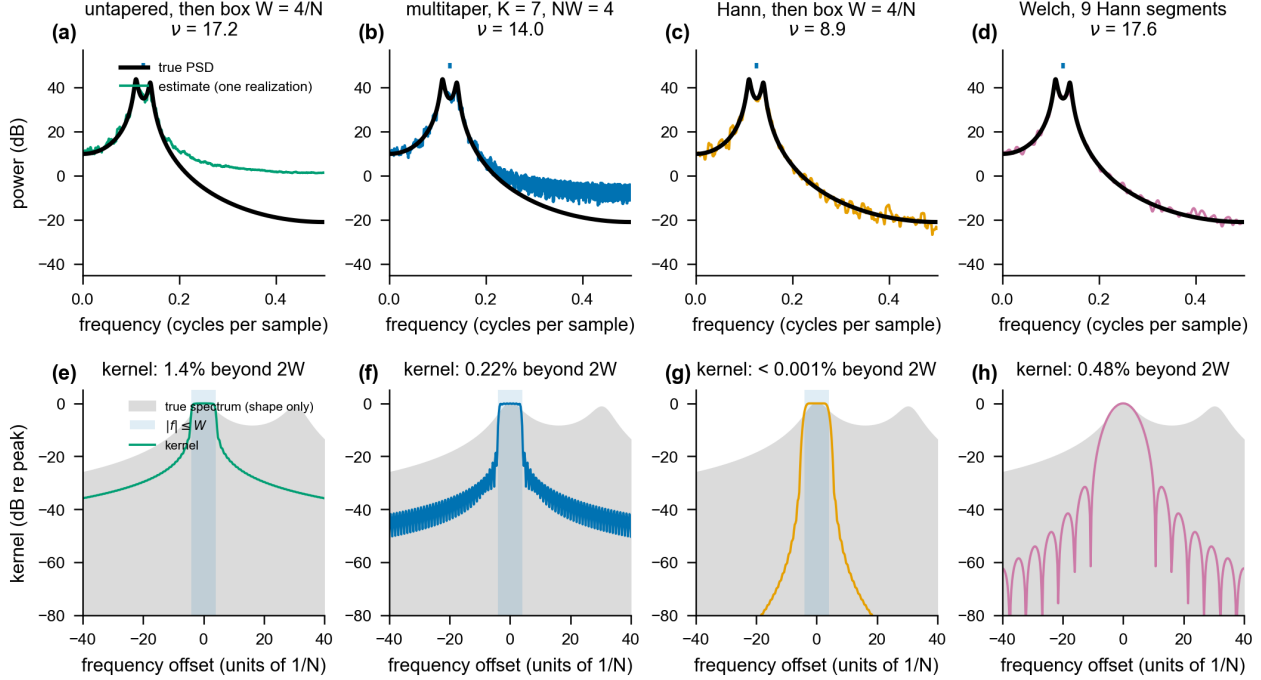
Figure 6: The estimators used in practice, applied to the record of Fig. 2 ( N = 1024 , W = 4/N ; one realization). (a–d) The untapered periodogram smoothed with a box, which is the exact estimate (7) (green); Thomson’s estimate with K = 7 tapers (blue); a Hann-tapered periodogram smoothed with the same box (orange); and Welch’s method with nine Hann segments of 192 samples stepped by 104, chosen for approximately the same half-power width (purple; the four widths are 8.2, 7.2, 8.2 and 7.8/ N ). This realization has more leakage than is typical. Its median absolute errors over the band are 11.6, 4.6, 1.3 and 0.8 dB, and the values over 300 realizations are 5.3, 2.3, 1.4 and 1.0 dB (Table 1). (e–h) The kernels, as in Fig. 2. The untapered box (e) inherits the Fejér tails, and its estimate levels off 20 dB above the true spectrum. The seventh Slepian taper puts the skirt of the multitaper kernel at -22 dB (f), and that estimate levels off 10 dB above the true spectrum. The Hann kernel (g) falls below -36 dB beyond the box. Welch’s kernel (h) has no flat top, and its side lobes are spaced at the scale of the peaks.
