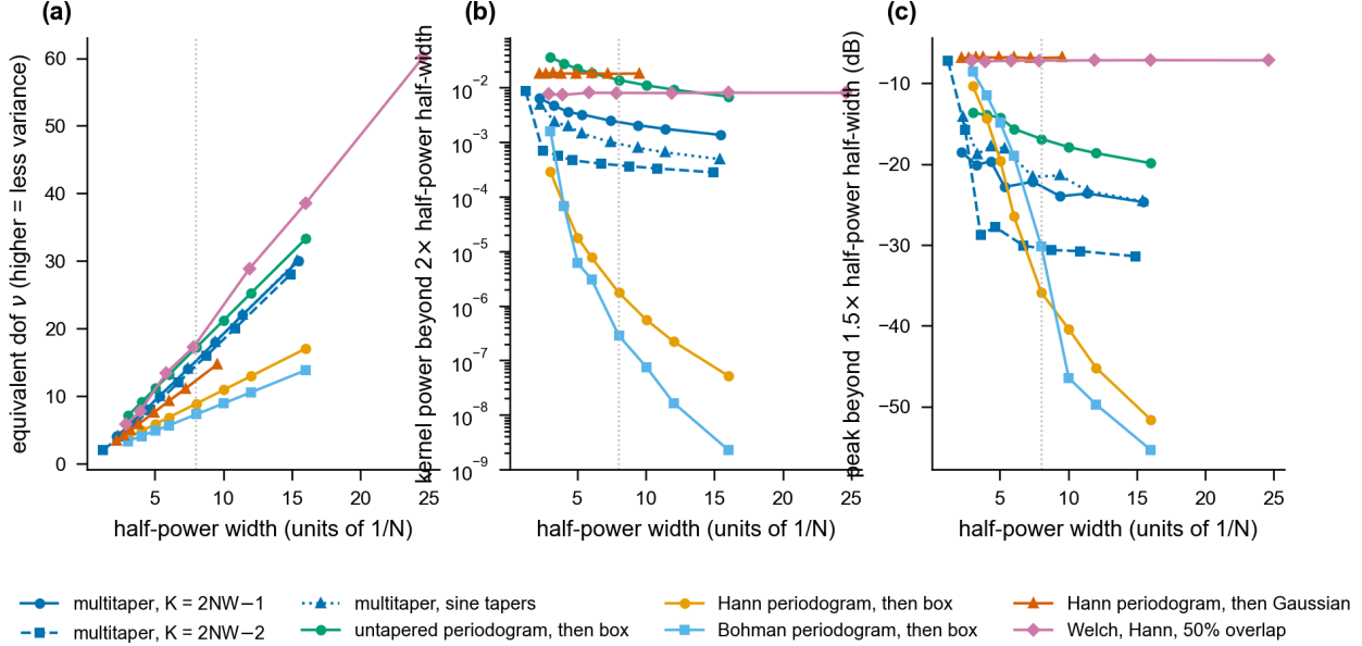
Figure S3: Variance, leakage and side-lobe level versus measured resolution for N = 256 . All curves are exact kernel and degrees-of-freedom computations, with no sampling variability. Each method's bandwidth parameter is swept and the quantities are plotted against the resulting half-power width, so methods are compared at equal resolution: multitaper with K = 2NW - 1 and 2NW - 2 Slepian tapers and with sine tapers; untapered, Hann and Bohman periodograms followed by a box; a Hann periodogram followed by a Gaussian; Welch's method with 50% overlap. (a) Equivalent degrees of freedom \nu (higher means less variance). (b) Kernel power beyond twice the half-power half-width. (c) The peak of the kernel beyond 1.5 \times the half-power half-width. The Gaussian and Welch kernels have no flat top, so for them this quantity is the skirt of the main lobe and not a side lobe. The dotted line marks the 8/N width of Table 2.
