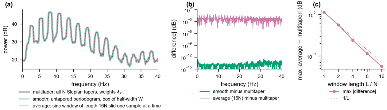
Figure 1: Three routes to one spectrum. (a) Power spectral density (PSD) of eight seconds of one channel of de-identified scalp EEG at 128 Hz from the authors’ archive ( N = 1024 ; one epoch), design half-bandwidth W = 4/N = 0.5 Hz, by three routes: the multitaper estimate with all N Slepian tapers weighted by their eigenvalues \lambda_k (thick grey); the untapered periodogram smoothed with a box of half-width W (green); and the average of periodograms of a sinc window of half-bandwidth W and length 16N slid across the record one sample at a time (dashed purple). (b) Absolute differences from the multitaper estimate on a logarithmic scale: the smoothed periodogram agrees to 3 \times 10^{-13} dB, the sliding-window average to 0.06 dB. (c) The maximum difference of the sliding-window average versus window length, with a 1/L guide line. The multitaper estimate here has \nu = 17 equivalent degrees of freedom, as defined in Section 2.
