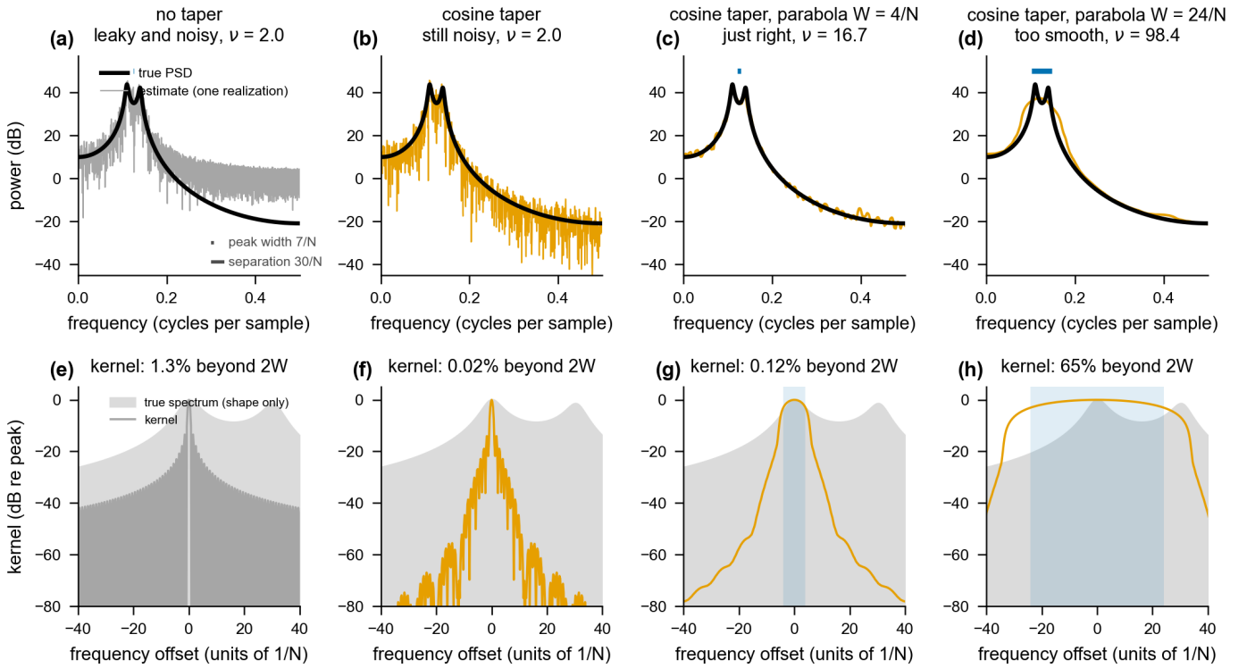
Fig. 2. Every estimator is the true spectrum blurred by a kernel, plus noise. (a–d) One realization ( N = 1024 ) of an autoregressive process whose PSD (black) has two peaks 7/N wide at half power and 30/N apart on a background spanning 65 dB, estimated by the periodogram (a), the periodogram of the record after a 25% cosine taper (b), the same smoothed with a parabola whose half-power width 2W = 8/N is that of a peak (c), and smoothed with 2W = 48/N , which exceeds the separation of the peaks (d). The short blue bar above the peaks is the half-power width of each estimator's kernel, and the grey bars in (a) mark the peak width and separation. The equivalent degrees of freedom are denoted \nu . (e–h) Each estimator's expected-value kernel in dB relative to its peak, drawn over the true spectrum around its peaks (grey, showing its shape only). Blue shading marks |f| \leq W . The panel titles give the fraction of the kernel's power outside |f| \leq 2W , which is our measure of broadband leakage. The skirts of the Fejér kernel fall slowly, so power leaks from the peaks into the region 40 dB below them (a, e). The cosine taper lowers the skirts by 22 dB at 16/N and by 39 dB at 40/N , and widens the main lobe by 15% (f). A kernel as wide as a peak is just right (g), and a wider kernel merges the peaks (h).
