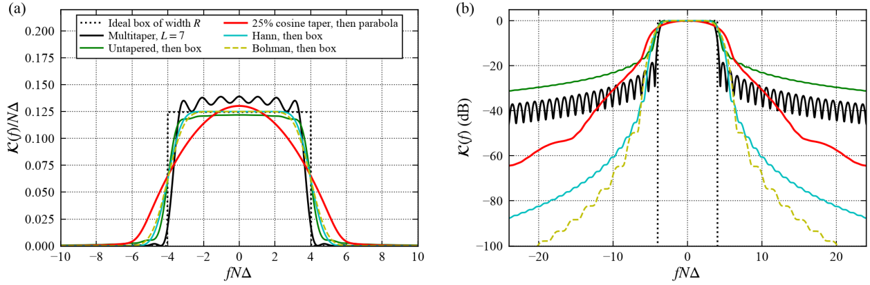
Figure S1. Kernels at the same design resolution ( N = 256 , R = 8/(N\Delta) ; Table 2), (a) on a linear scale near the main lobe and (b) in dB relative to the peak: the ideal box (dotted); the L = 7 multitaper kernel ( \nu = 14.0 , black); the periodogram after a 25% cosine taper followed by a parabola of the same half-power width ( \nu = 16.7 , red), which is recipe (b’); and the untapered ( \nu = 17.2 , green), Hann ( \nu = 8.9 , cyan) and Bohman ( \nu = 7.3 , olive, dashed) periodograms followed by the box. All main lobes have nearly the same half-power width, and the skirts differ by 40 dB.
