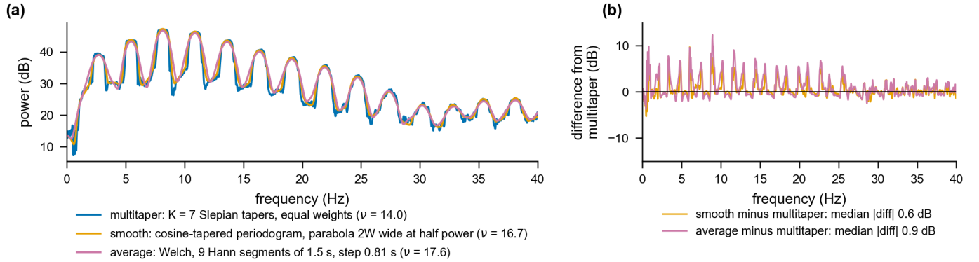
Fig. 7. The estimators used in practice agree to within their own noise. (a) The EEG epoch of Fig. 1 estimated by Thomson's method with K = 7 tapers ( \nu = 14 , blue); by a cosine-tapered periodogram smoothed with a parabola of half-power width 2W ( \nu = 16.7 , orange); and by Welch's method with nine Hann segments of 1.5 s stepped by 0.81 s ( \nu = 17.6 , purple). Their half-power widths are 0.91, 1.03 and 0.97 Hz. (b) Differences from the multitaper estimate: median absolute difference 0.6 dB (smoothed) and 0.9 dB (averaged), 95th percentiles 4.2 and 5.9 dB. The medians are smaller than the estimators' own noise ( 4.3\sqrt{2/\nu} gives 1.6, 1.5 and 1.5 dB). The largest differences are in the valleys between harmonics, which the seventh Slepian taper's side lobes fill in.
