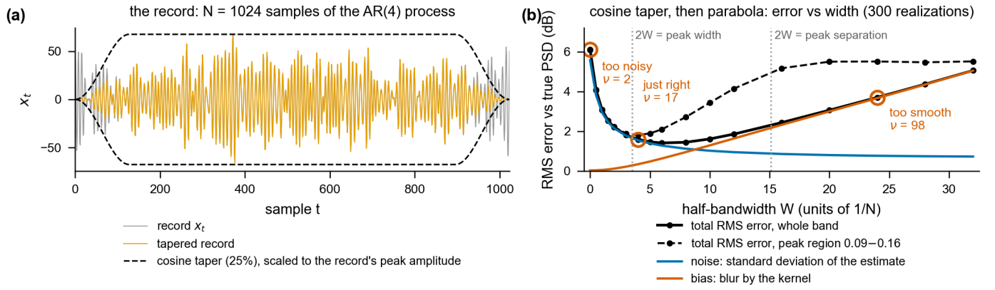
Fig. 3. Choosing the bandwidth. (a) The record of Fig. 2: N = 1024 samples of the AR(4) process (grey), the 25% cosine taper scaled to the record's peak amplitude (dashed), and the tapered record (orange). (b) Root-mean-square error over frequency, in dB, of the cosine-tapered periodogram smoothed with a parabola of half-power width 2W , against the true PSD as W varies, averaged over 300 independent realizations; no error bars are shown because the curves are ensemble averages. Noise (the standard deviation of the estimate, blue) falls with W , blur (the bias of the kernel, orange) grows, and their total (black) has a broad minimum that sits at smaller W when only the peak region, 0.09 to 0.16 cycles per sample, is scored (dashed). The circled points are panels (b), (c) and (d) of Fig. 2.
