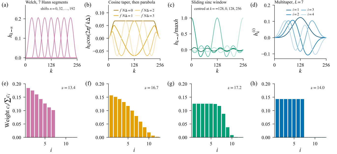
Figure 5: Three ways to build a bank of tapers from one window, and the reference bank ( N = 256 , R = 8/(N\Delta) , \alpha = 4 ). Every curve and weight is computed exactly. (a–d) The bank as constructed, in one colour for each route, with lighter shades for later members of the bank in (b–d). (a) Welch’s method with Hann segments of length N/4 at 50% overlap: seven time-shifted copies of one window. (b) A periodogram tapered with a 25% cosine taper and smoothed with a parabola of half-power width R : frequency-shifted copies of one taper, four of a continuum. (c) A sinc window of bandwidth R slid across the record one sample at a time, four positions shown; in the limit of a long window this is exactly the untapered periodogram smoothed with a box, and exactly Thomson’s estimate with all N tapers weighted by \lambda_i . (d) Thomson’s estimate with L = 7 equally weighted Slepian tapers, the first four shown. (e–h) The eigen-weight ladder c_i of each, normalized to unit sum, whose flatness sets \nu = 2(\sum_i c_i)^2 / \sum_i c_i^2 by (15): \nu = 13.4 , 16.7 , 17.2 and 14.0 . The eigen-tapers of (c) are the Slepian sequences themselves. Fig. S1 adds the eigen-tapers and kernels.
