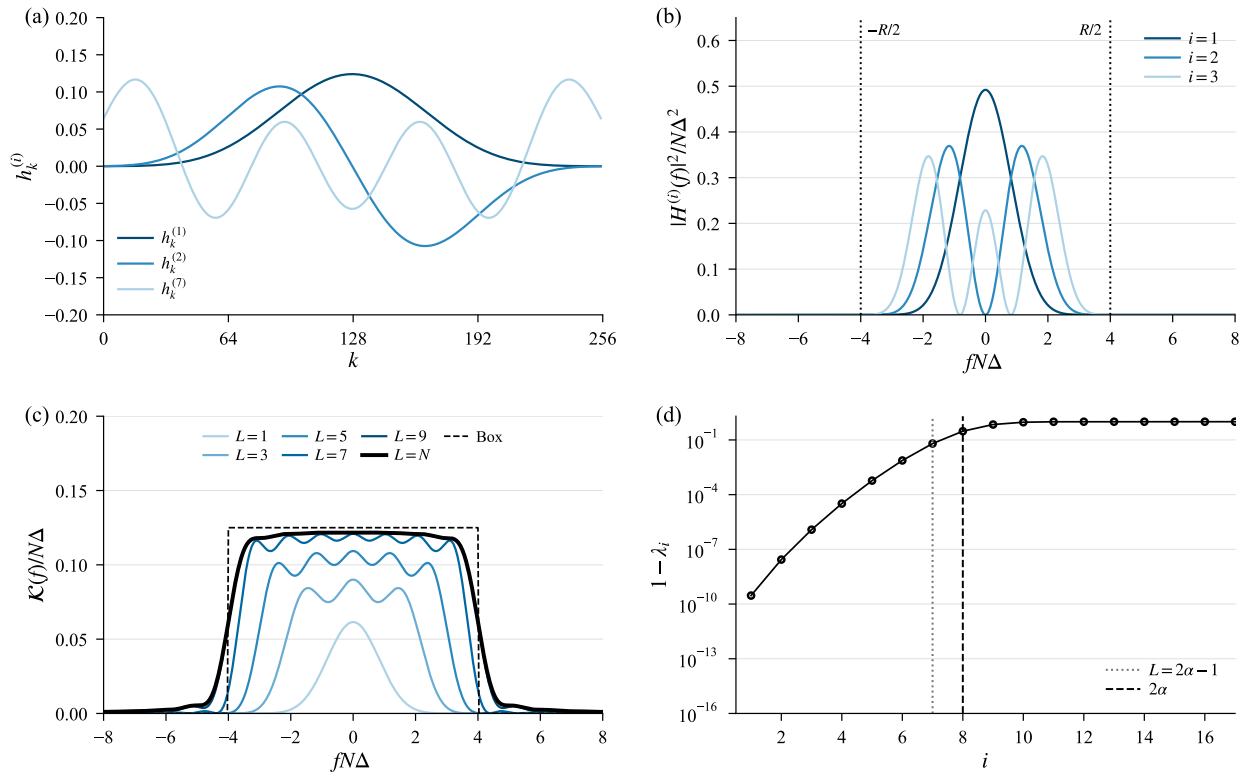
Figure 4: Why the multitaper kernel is a box ( N = 256 , R = 8/(N\Delta) , \alpha = 4 ). Every curve is computed exactly, and nothing is simulated. (a) The first, second and seventh Slepian tapers, from dark to light. (b) The kernels |H^{(i)}(f)|^2/\Delta of the first three, in units of N\Delta , each filling the gaps left by the previous ones within the band |f| \leq R/2 (dotted lines). (c) The running sum \sum_{i \leq L} \lambda_i |H^{(i)}(f)|^2/2\alpha\Delta as tapers are added, in the same units and darker for larger L . With all N tapers it is exactly the box of width R (dashed) convolved with Fejér’s kernel, which is the identity (16) in kernel form. For this short record the convolution rounds the edges of the box over about 1/(N\Delta) on each side and lowers its top by 3%. With the usual L = 2\alpha - 1 = 7 it is the box with rounded shoulders and small ripple. (d) The concentration ladder: the fraction 1 - \lambda_i of each taper’s energy outside the band. Tapers beyond the 2\alpha th carry only leakage.
