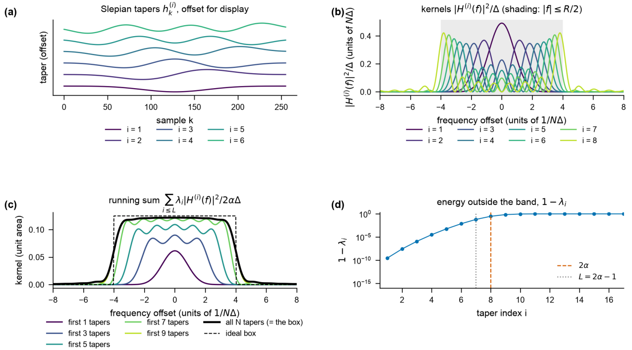
Fig. 4. Why the multitaper kernel is a box. N = 256 , R = 8/(N\Delta) . (a) The first six Slepian tapers h^{(i)} , offset vertically for display. (b) Their kernels |H^{(i)}(f)|^2/\Delta , each filling the gaps left by the previous ones within the band (shading: |f| \leq R/2 ). (c) The running sum \sum_{i \leq L} \lambda_i |H^{(i)}(f)|^2/2\alpha\Delta as tapers are added. With all N tapers it is exactly the box of width R convolved with Fejér's kernel, which is the identity (16) in kernel form and cannot be distinguished from the box itself (dashed) at this scale. With the usual L = 2\alpha - 1 = 7 it is the box with rounded shoulders and small ripple. (d) The concentration ladder: the fraction 1 - \lambda_i of each taper's energy outside the band. Tapers beyond the 2\alpha th carry only leakage.
