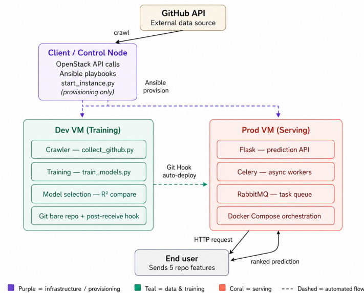
Figure 1: Distributed ML system: Data collection and training on Dev VM, deployment via Git Hook, serving on Prod VM with Flask + Celery + RabbitMQ.
