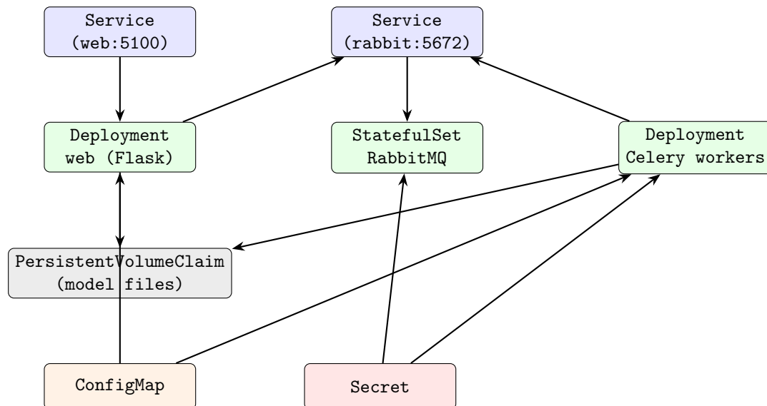
Figure 7: Kubernetes deployment diagram: Flask web Deployment behind a Service, RabbitMQ StatefulSet with headless Service, Celery worker Deployment, shared PersistentVolumeClaim for model files, ConfigMap and Secret for configuration and credentials.
