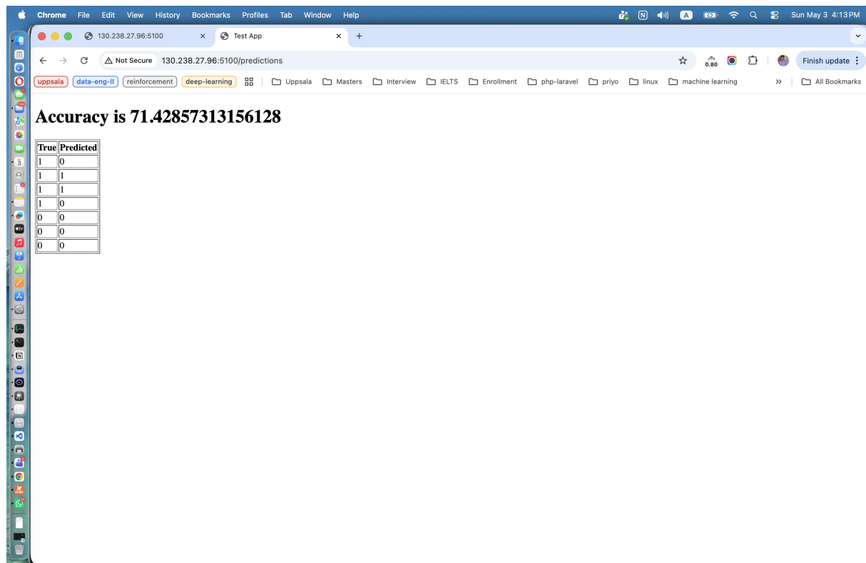
Figure 6: Predictions page reflecting the updated model after the CI/CD push.
