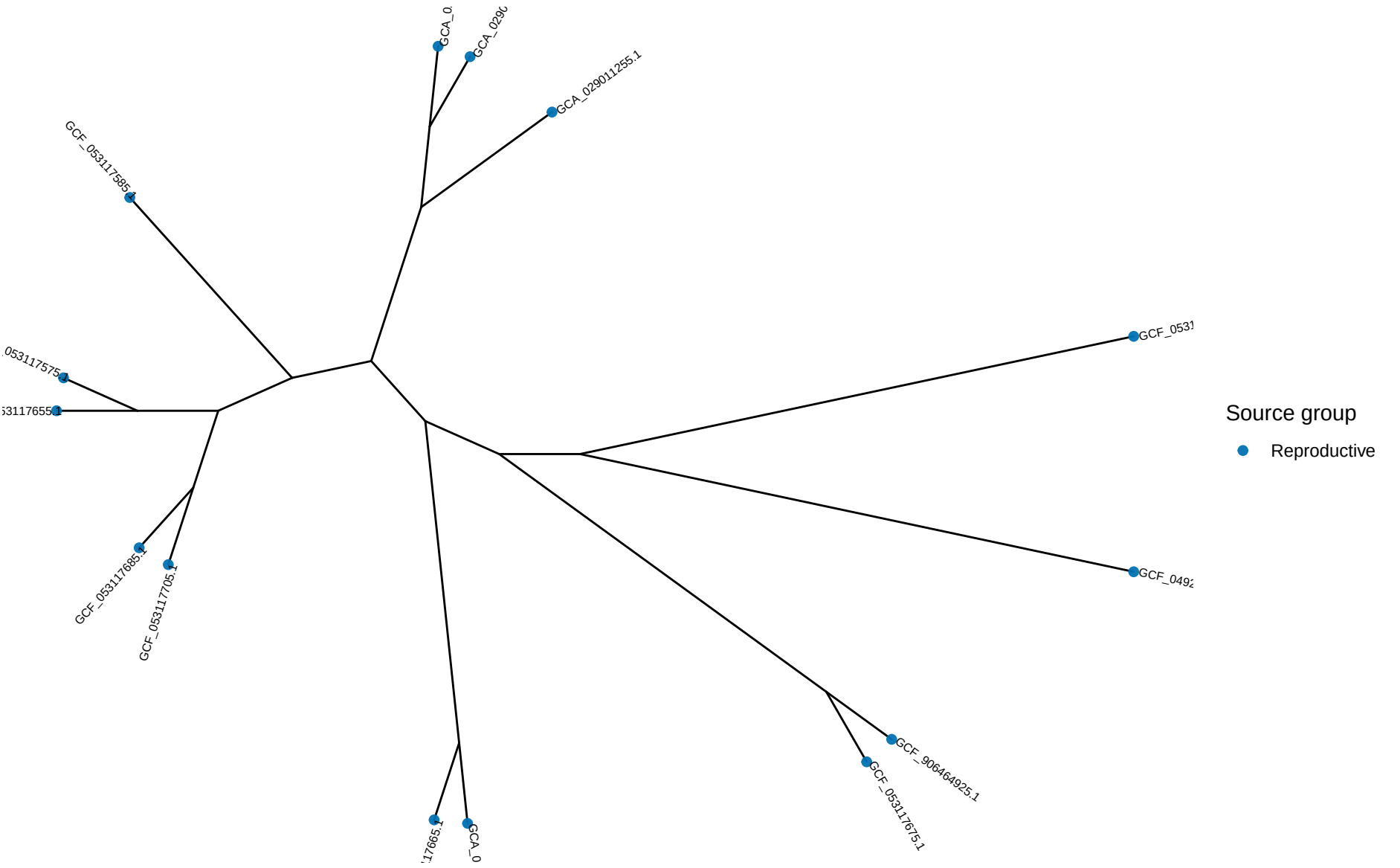
reproductive_14_pruned_unrooted_cladogram Pruned from 72-tip ML tree, topology-only (branch-length scaling suppressed)
