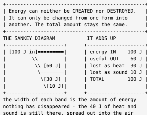
*Fig. 3: The law of conservation of energy*
