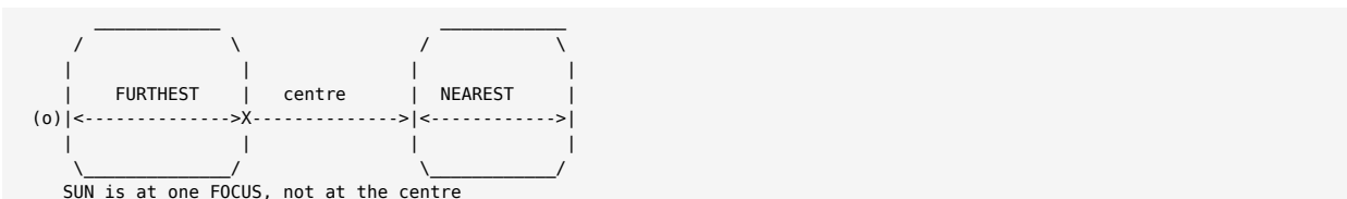
*Fig. 6: An elliptical orbit*
