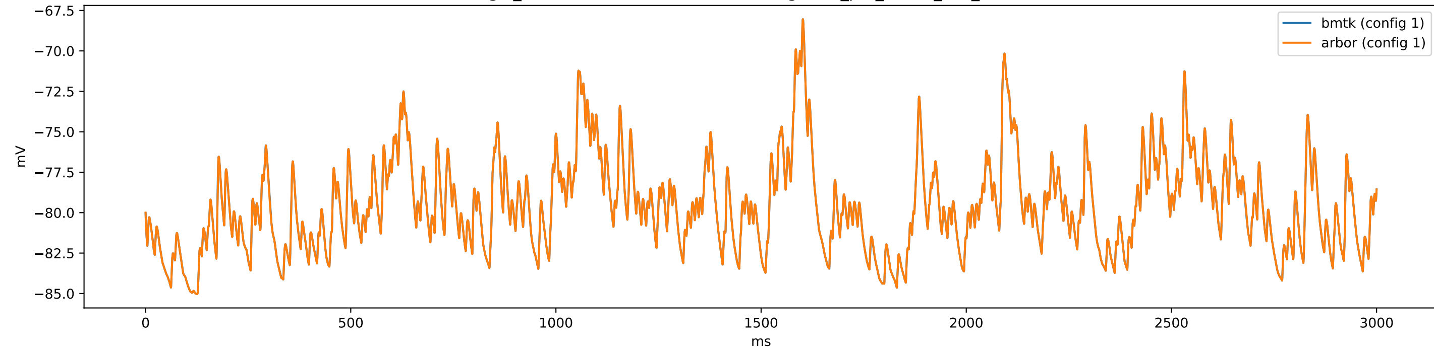
gid_102-471789504 (e6Ntsr1) - config.1cell_per_model_dL5_iclamp
