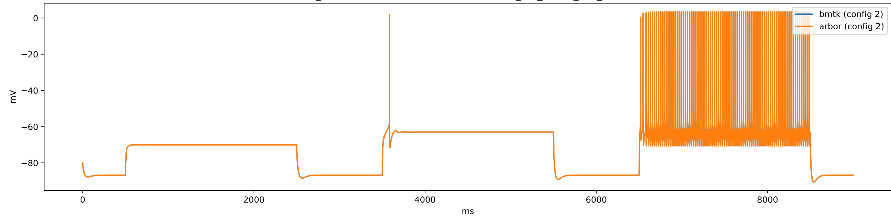
gid_12-484635029 (i23Pvalb) - config.1cell_per_model_dL5_iclamp
