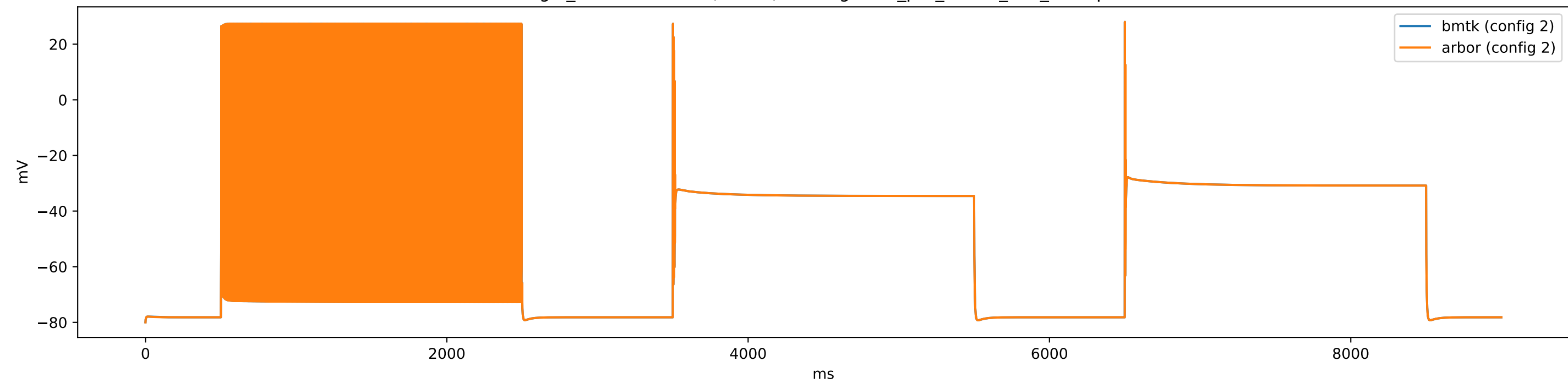
gid_17-476686112 (i23Sst) - config.1cell_per_model_dL5_iclamp
