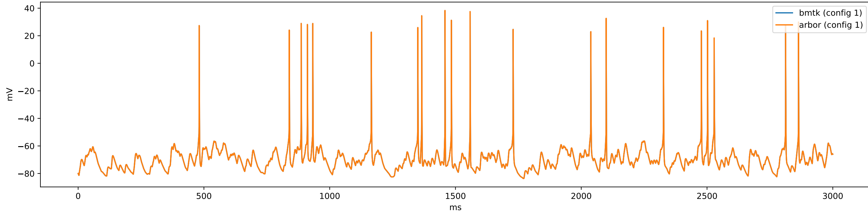
gid_19-318808427 (e4Nr5a1) - config.1cell_per_model_dL5_iclamp
