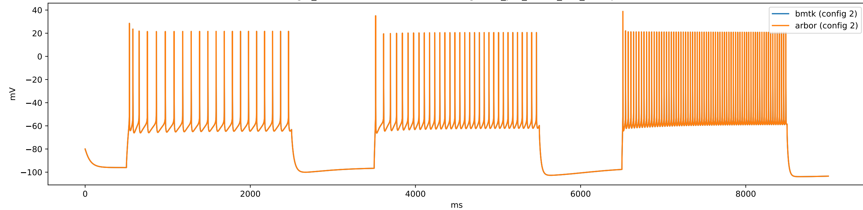
gid_2-487661754 (e23Cux2) - config.1cell_per_model_dL5_iclamp
