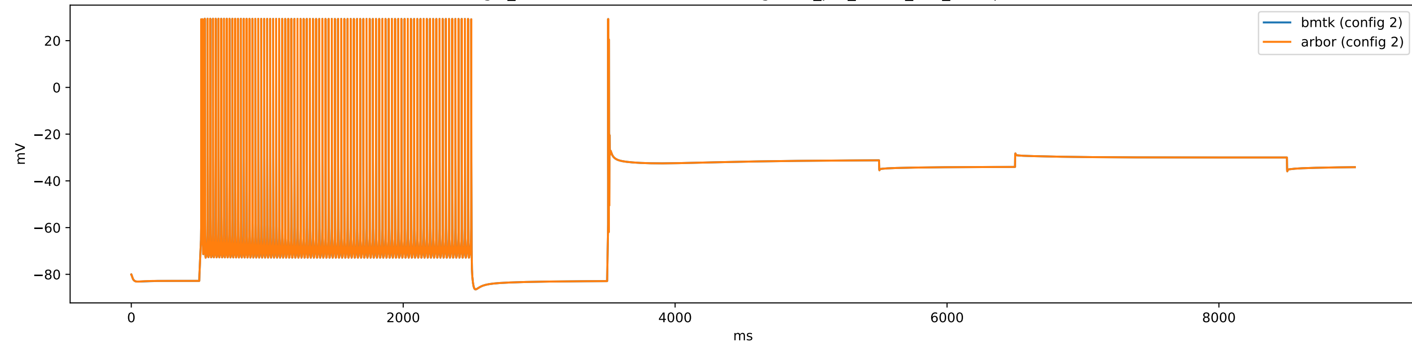
gid_31-476616076 (e4Rorb) - config.1cell_per_model_dL5_iclamp
