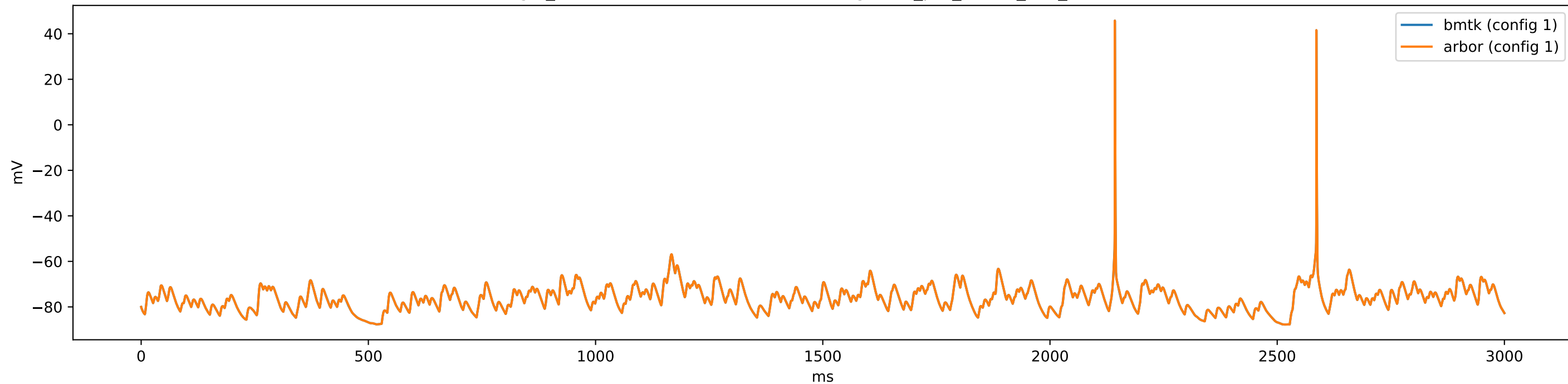
gid_43-476218657 (e4Scnn1a) - config.1cell_per_model_dL5_iclamp
