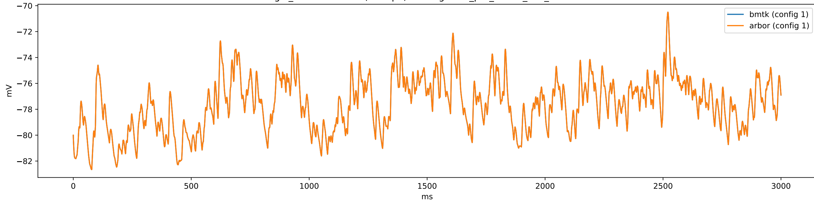
gid_59-485835055 (e5Rbp4) - config.1cell_per_model_dL5_iclamp
