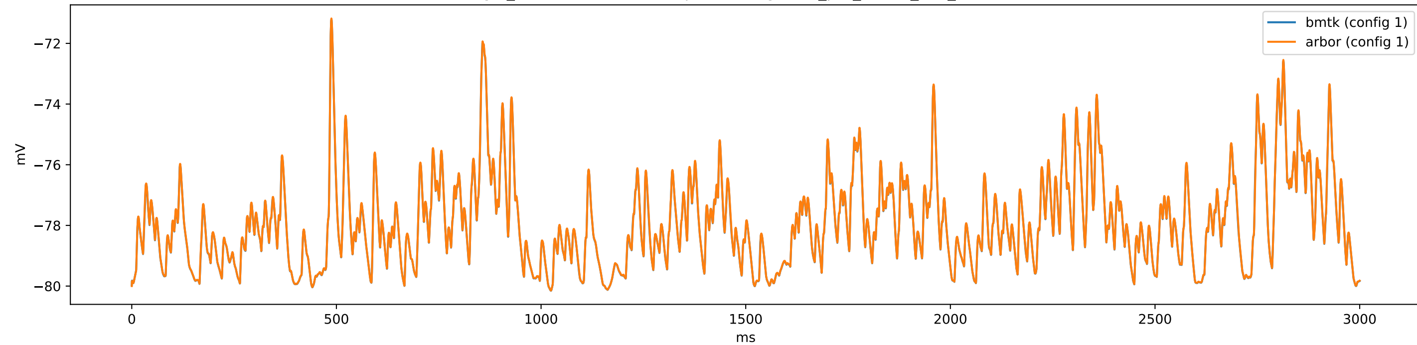
gid_61-486052980 (e5Rbp4) - config.1cell_per_model_dL5_iclamp
