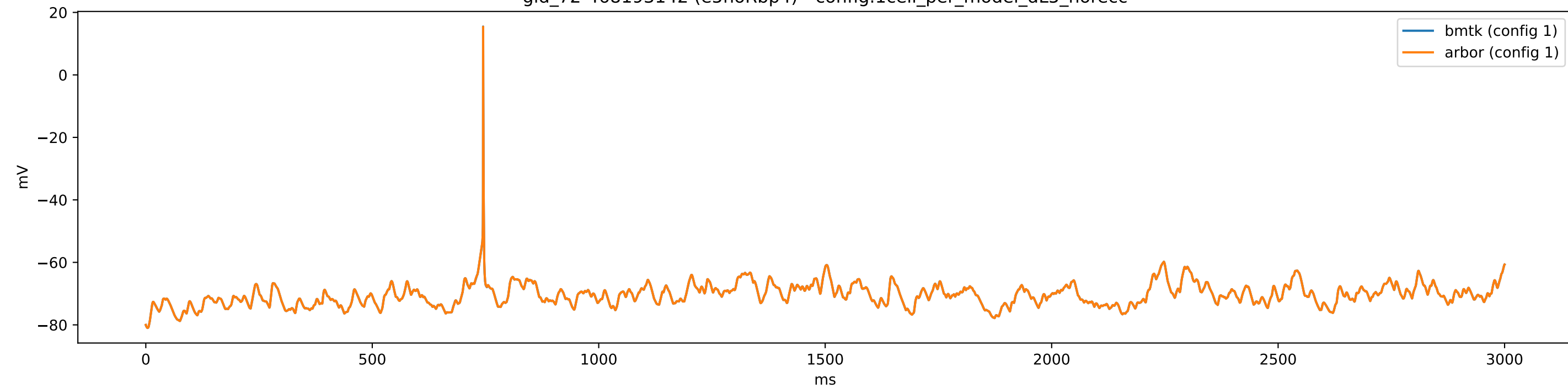
gid_72-468193142 (e5noRbp4) - config.1cell_per_model_dL5_iclamp
