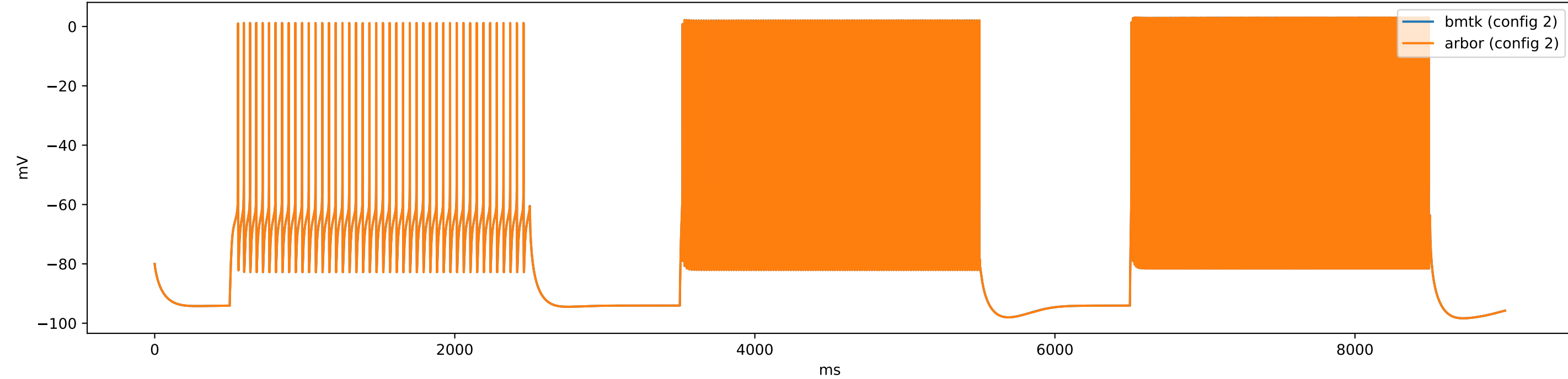
gid_89-469610831 (i5Pvalb) - config.1cell_per_model_dL5_iclamp
