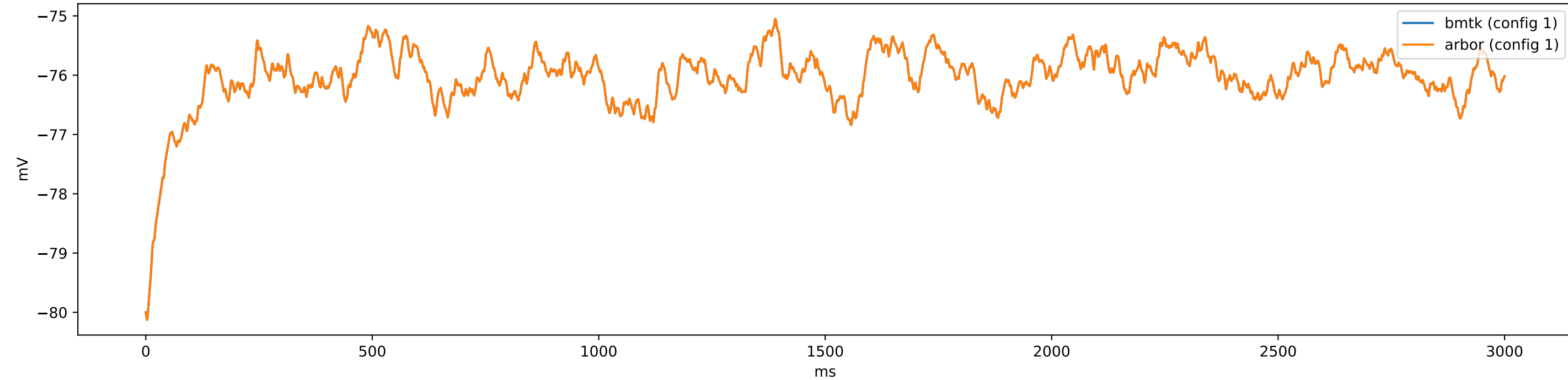
gid_97-478396248 (i5Sst) - config.1cell_per_model_dL5_iclamp
