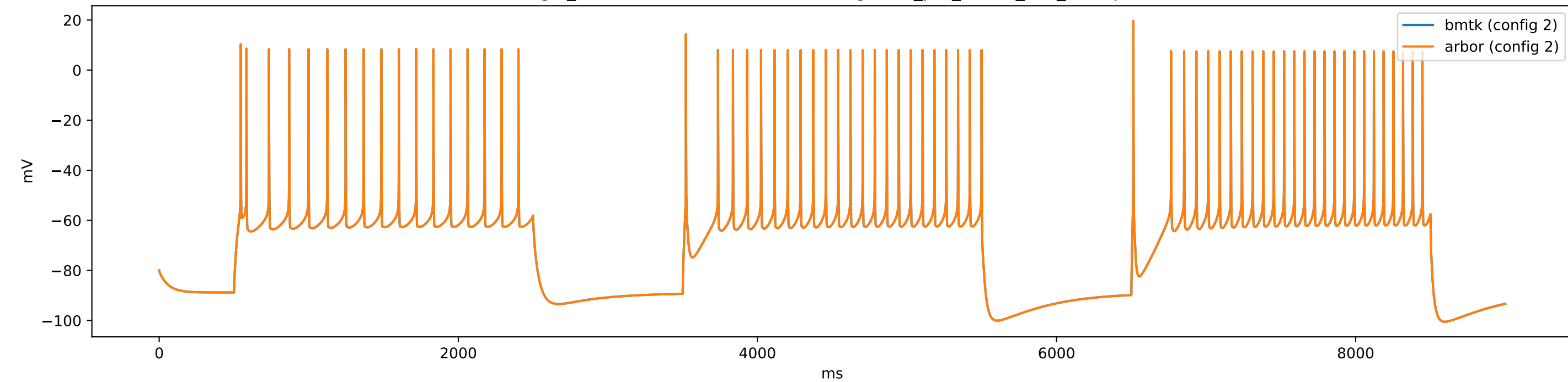
gid_99-466632464 (e6Ntsr1) - config.1cell_per_model_dL5_iclamp
