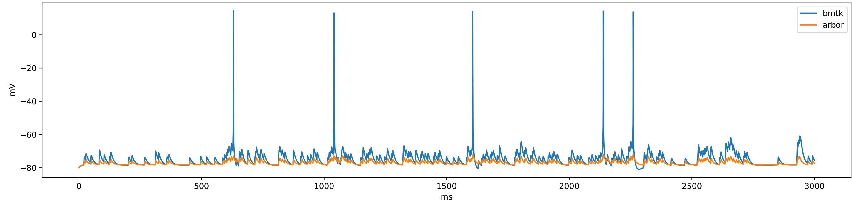
478107198 (i1Htr3a)
