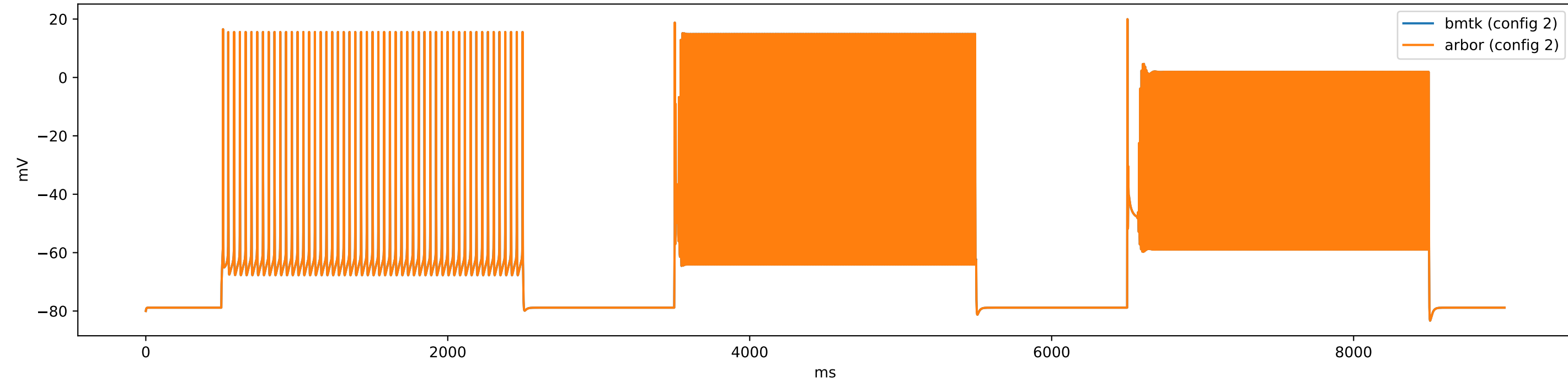
gid_0-475585413 (i1Htr3a) - config.1cell_per_model_iclamp
