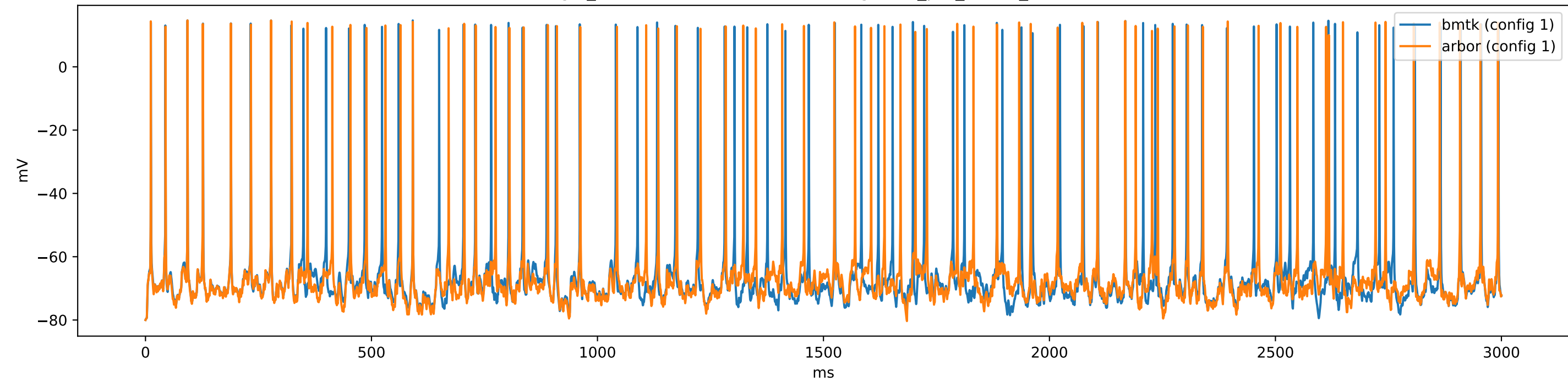
gid_1-478107198 (i1Htr3a) - config.1cell_per_model_iclamp
