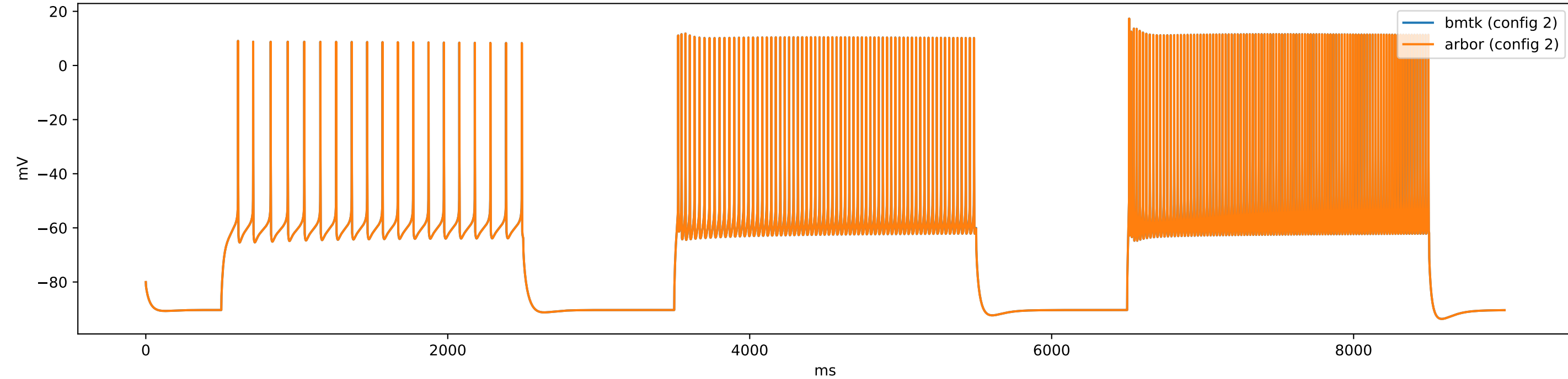
gid_100-471410185 (e6Ntsr1) - config.1cell_per_model_iclamp
