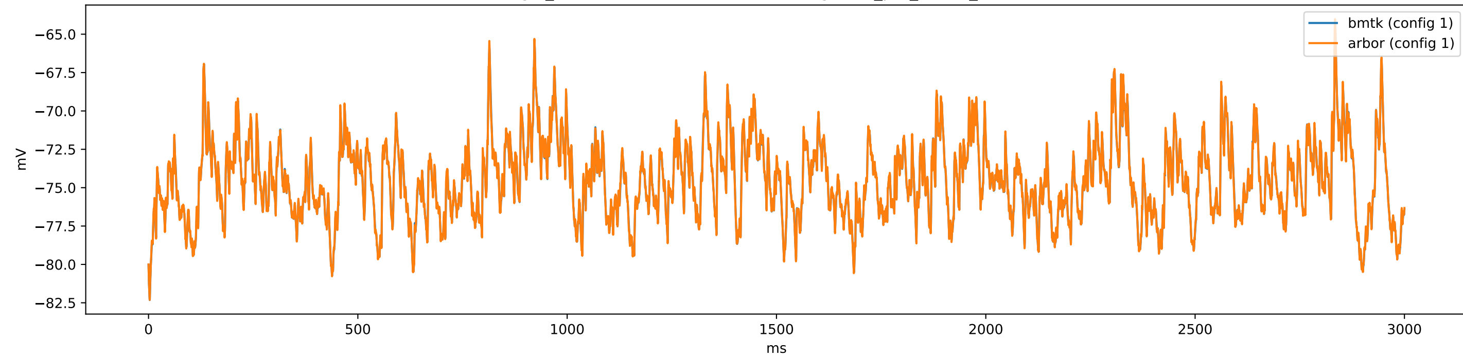
gid_106-321708130 (i6Pvalb) - config.1cell_per_model_iclamp
